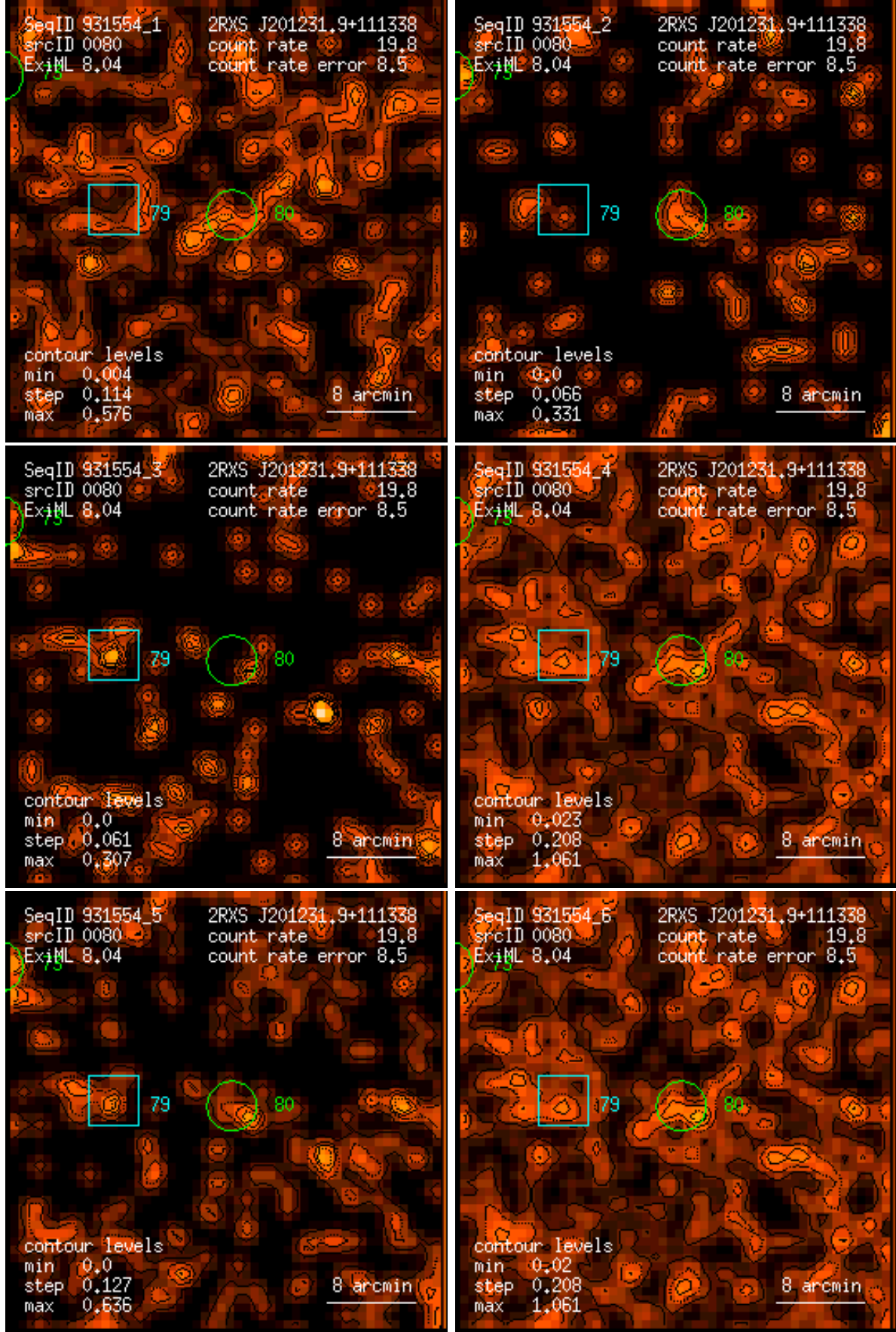
Figure 80: RASS 931554: detection 0080: band rate images, Gaussian filter: (1) PSPC channels 11 – 41, (2) 52 – 90, (3) 91 – 201, (4) 11 – 235, (5) 52 – 201, (6) 11 – 201. Broad band rates in counts/ks. Band rate contour levels in counts/ks/arcmin 2 .
