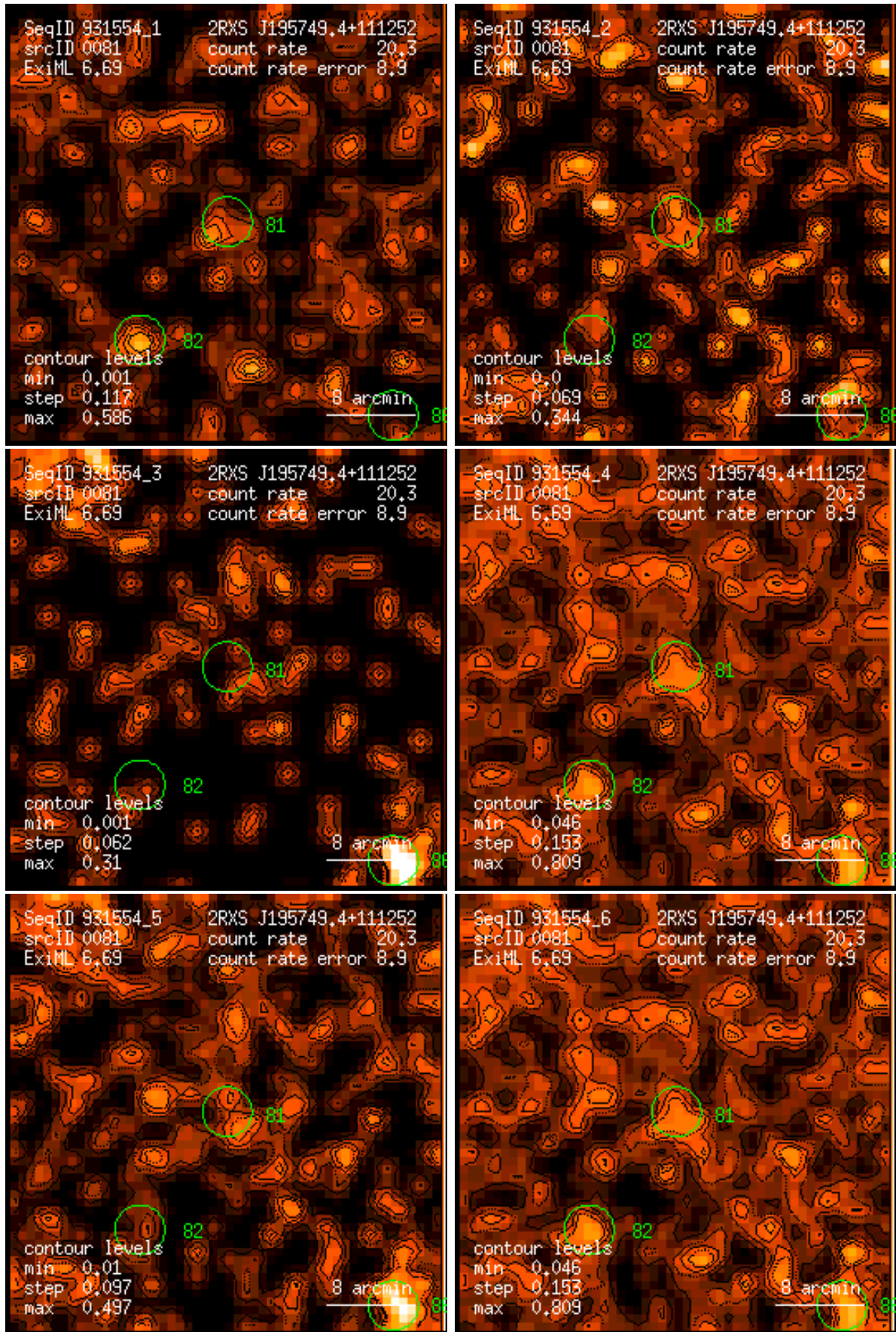
Figure 81: RASS 931554: detection 0081: band rate images, Gaussian filter: (1) PSPC channels 11 – 41, (2) 52 – 90, (3) 91 – 201, (4) 11 – 235, (5) 52 – 201, (6) 11 – 201. Broad band rates in counts/ks. Band rate contour levels in counts/ks/arcmin 2 .
