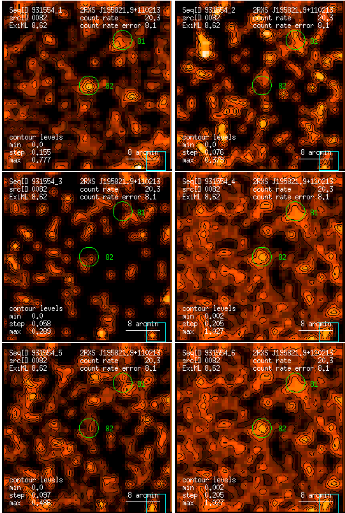
Figure 82: RASS 931554: detection 0082: band rate images, Gaussian filter: (1) PSPC channels 11 – 41, (2) 52 – 90, (3) 91 – 201, (4) 11 – 235, (5) 52 – 201, (6) 11 – 201. Broad band rates in counts/ks. Band rate contour levels in counts/ks/arcmin 2 .
