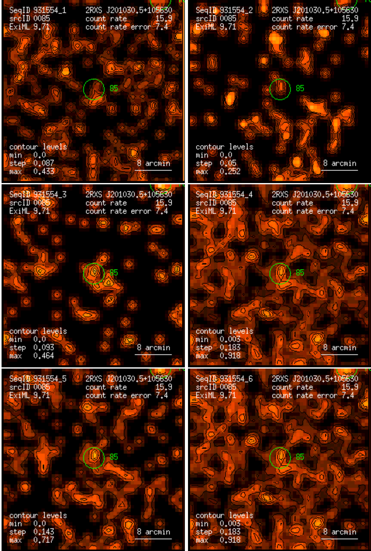
Figure 85: RASS 931554: detection 0085: band rate images, Gaussian filter: (1) PSPC channels 11 – 41, (2) 52 – 90, (3) 91 – 201, (4) 11 – 235, (5) 52 – 201, (6) 11 – 201. Broad band rates in counts/ks. Band rate contour levels in counts/ks/arcmin 2 .
