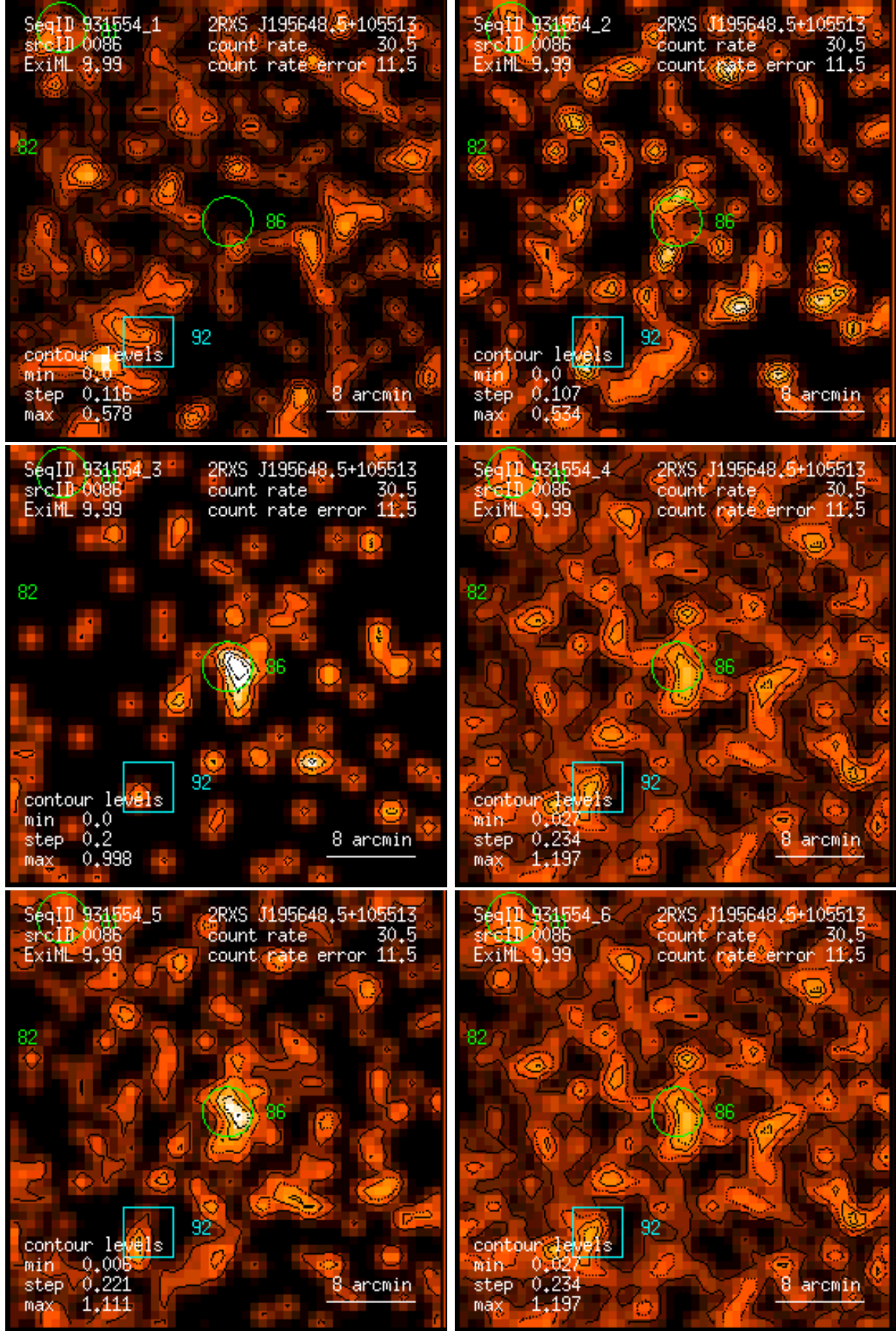
Figure 86: RASS 931554: detection 0086: band rate images, Gaussian filter: (1) PSPC channels 11 – 41, (2) 52 – 90, (3) 91 – 201, (4) 11 – 235, (5) 52 – 201, (6) 11 – 201. Broad band rates in counts/ks. Band rate contour levels in counts/ks/arcmin 2 .
