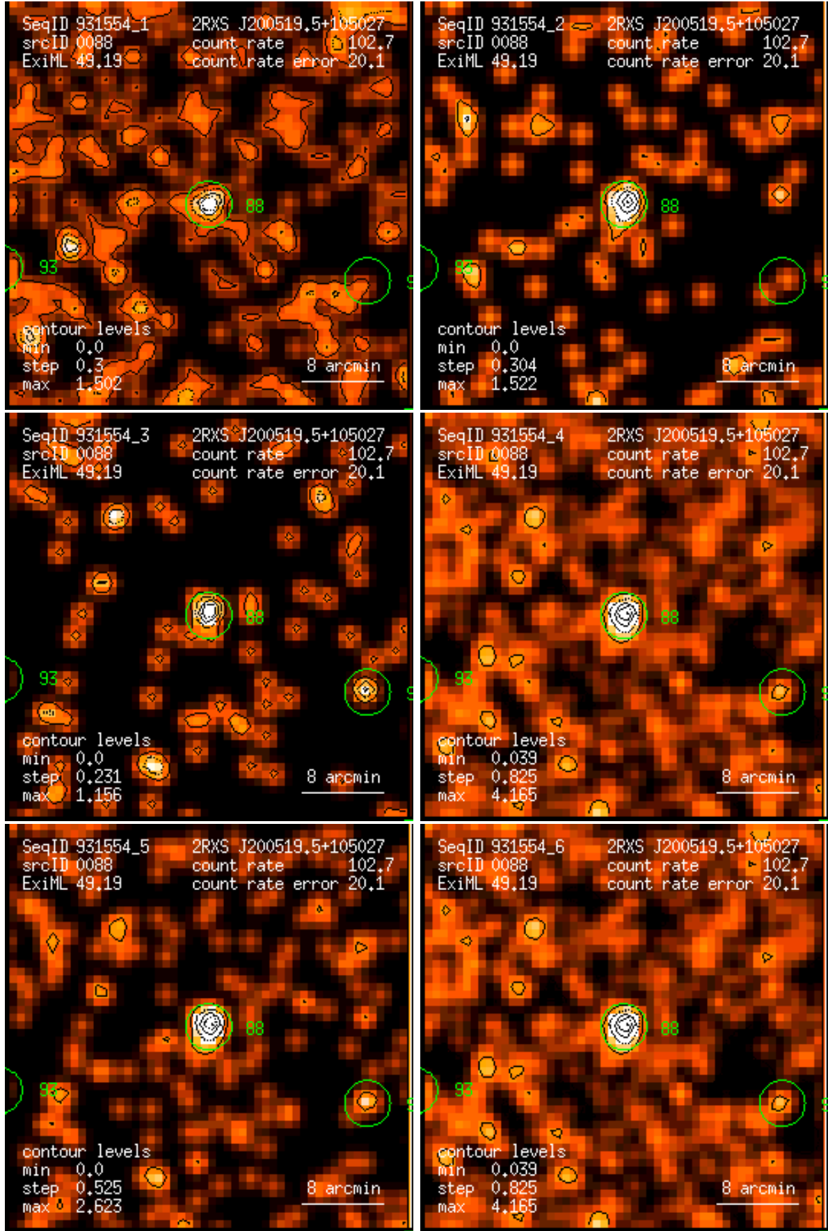
Figure 88: RASS 931554: detection 0088: band rate images, Gaussian filter: (1) PSPC channels 11 – 41, (2) 52 – 90, (3) 91 – 201, (4) 11 – 235, (5) 52 – 201, (6) 11 – 201. Broad band rates in counts/ks. Band rate contour levels in counts/ks/arcmin 2 .
