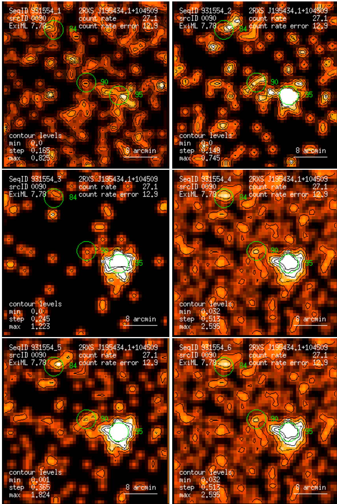
Figure 90: RASS 931554: detection 0090: band rate images, Gaussian filter: (1) PSPC channels 11 – 41, (2) 52 – 90, (3) 91 – 201, (4) 11 – 235, (5) 52 – 201, (6) 11 – 201. Broad band rates in counts/ks. Band rate contour levels in counts/ks/arcmin 2 .
