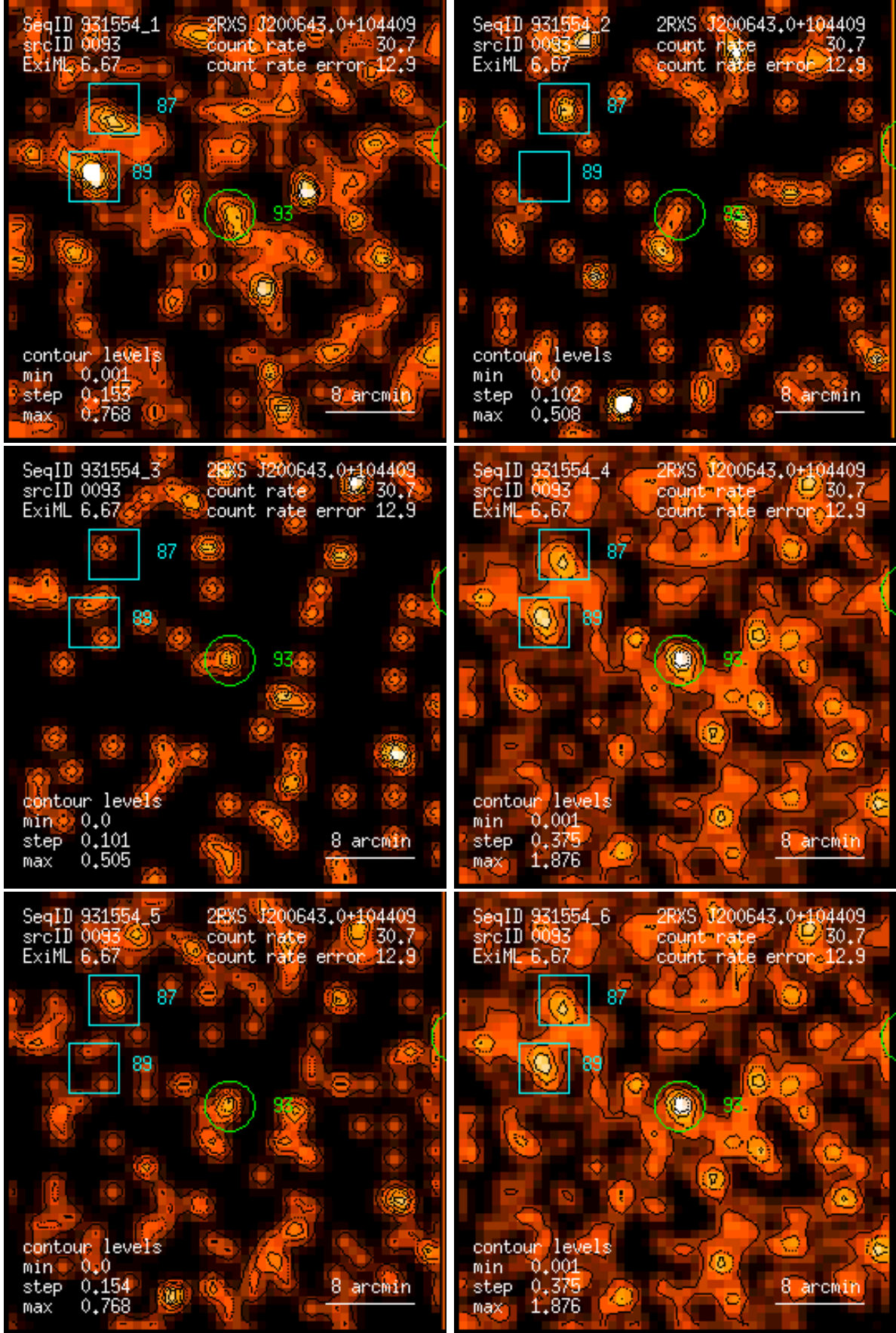
Figure 93: RASS 931554: detection 0093: band rate images, Gaussian filter: (1) PSPC channels 11 – 41, (2) 52 – 90, (3) 91 – 201, (4) 11 – 235, (5) 52 – 201, (6) 11 – 201. Broad band rates in counts/ks. Band rate contour levels in counts/ks/arcmin 2 .
