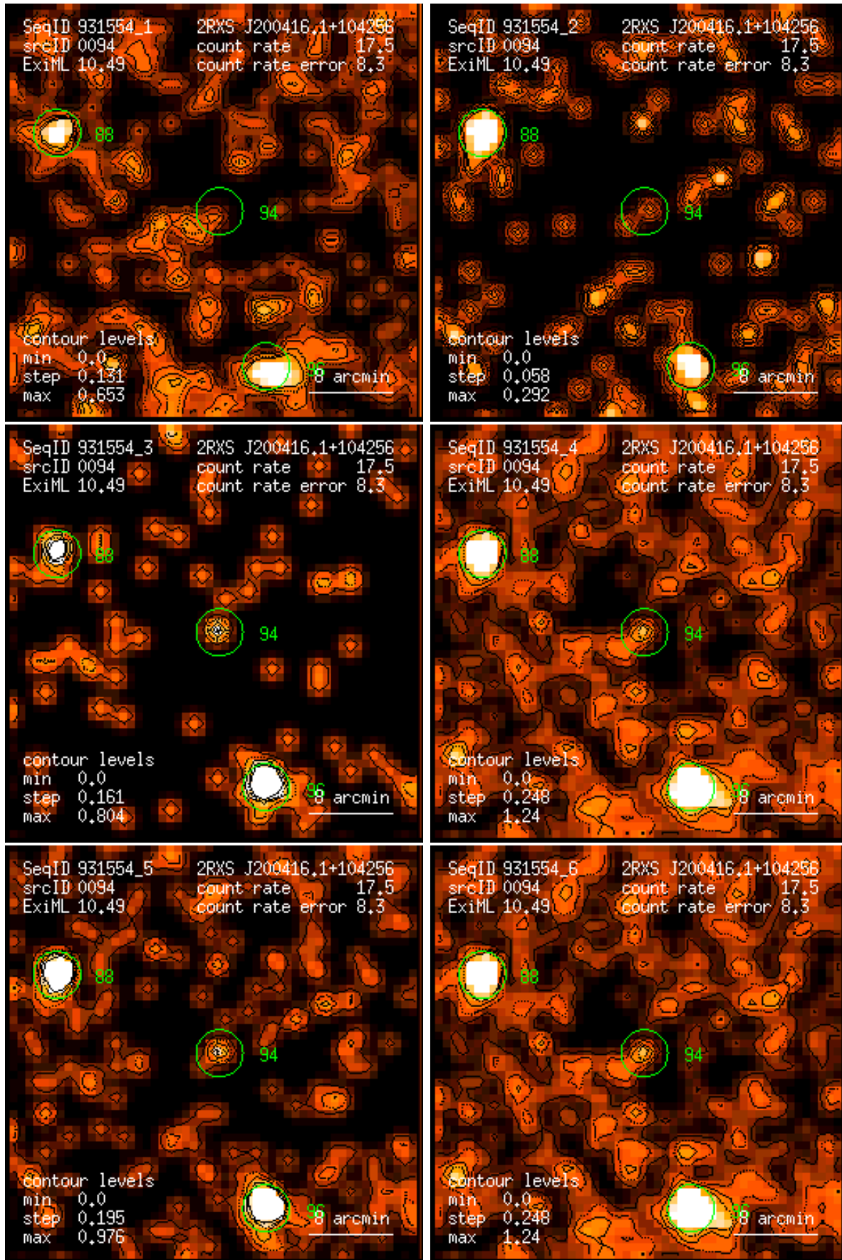
Figure 94: RASS 931554: detection 0094: band rate images, Gaussian filter: (1) PSPC channels 11 – 41, (2) 52 – 90, (3) 91 – 201, (4) 11 – 235, (5) 52 – 201, (6) 11 – 201. Broad band rates in counts/ks. Band rate contour levels in counts/ks/arcmin 2 .
