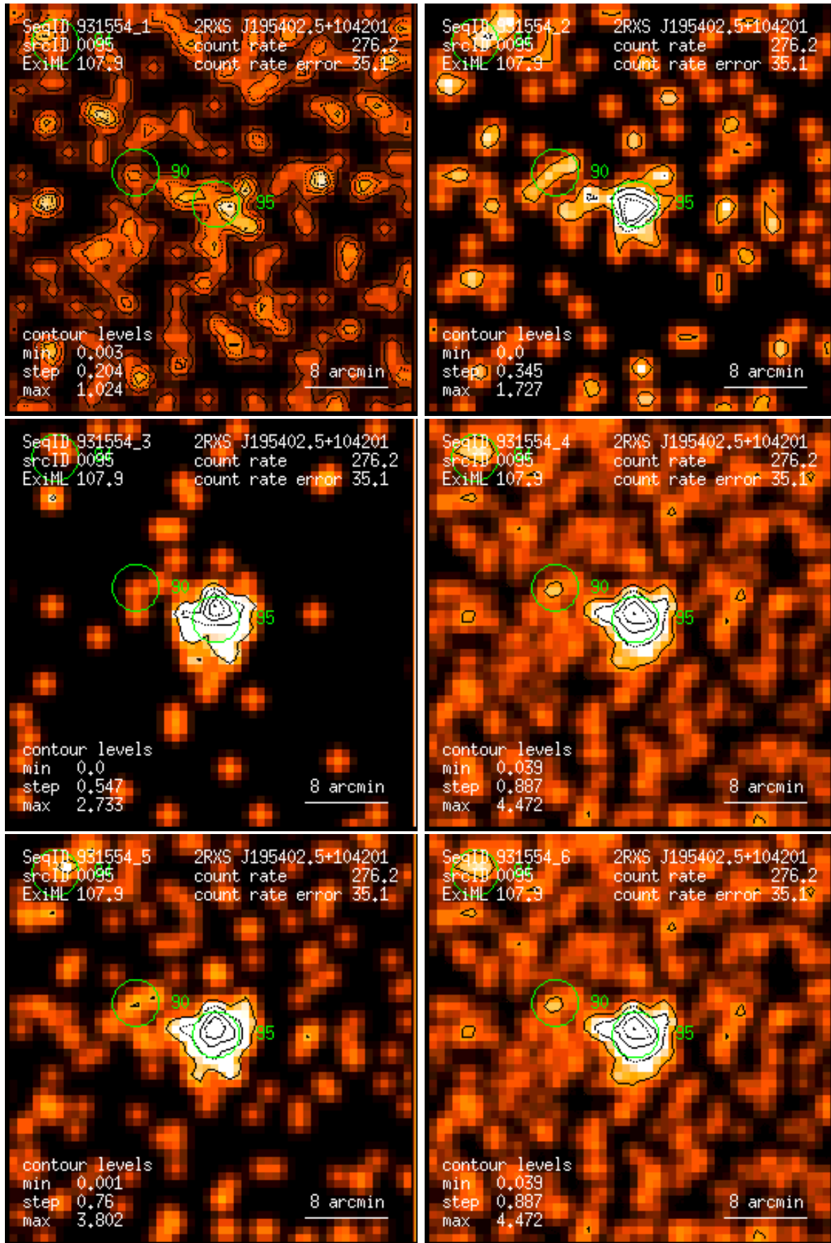
Figure 95: RASS 931554: detection 0095: band rate images, Gaussian filter: (1) PSPC channels 11 – 41, (2) 52 – 90, (3) 91 – 201, (4) 11 – 235, (5) 52 – 201, (6) 11 – 201. Broad band rates in counts/ks. Band rate contour levels in counts/ks/arcmin 2 .
