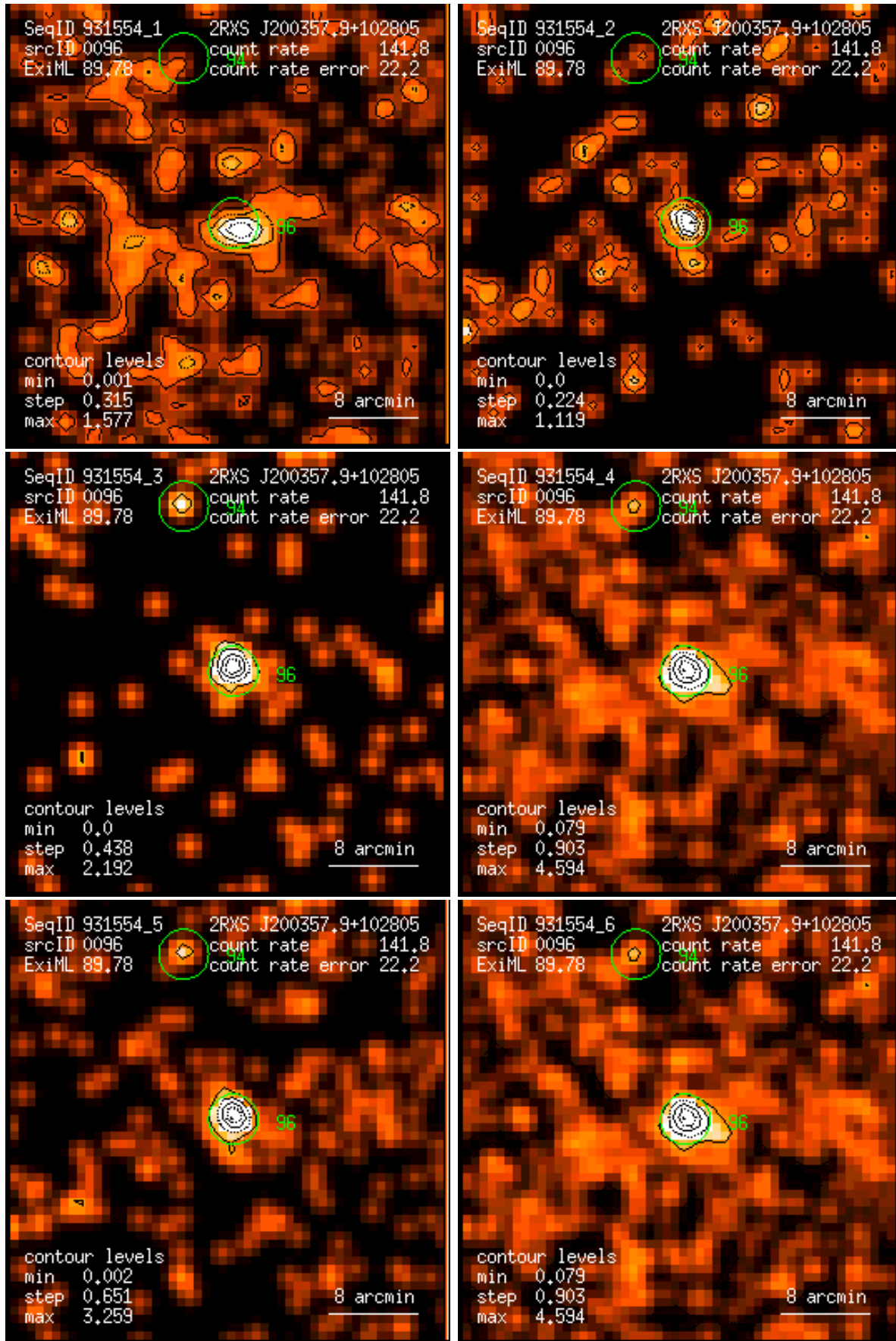
Figure 96: RASS 931554: detection 0096: band rate images, Gaussian filter: (1) PSPC channels 11 – 41, (2) 52 – 90, (3) 91 – 201, (4) 11 – 235, (5) 52 – 201, (6) 11 – 201. Broad band rates in counts/ks. Band rate contour levels in counts/ks/arcmin 2 .
