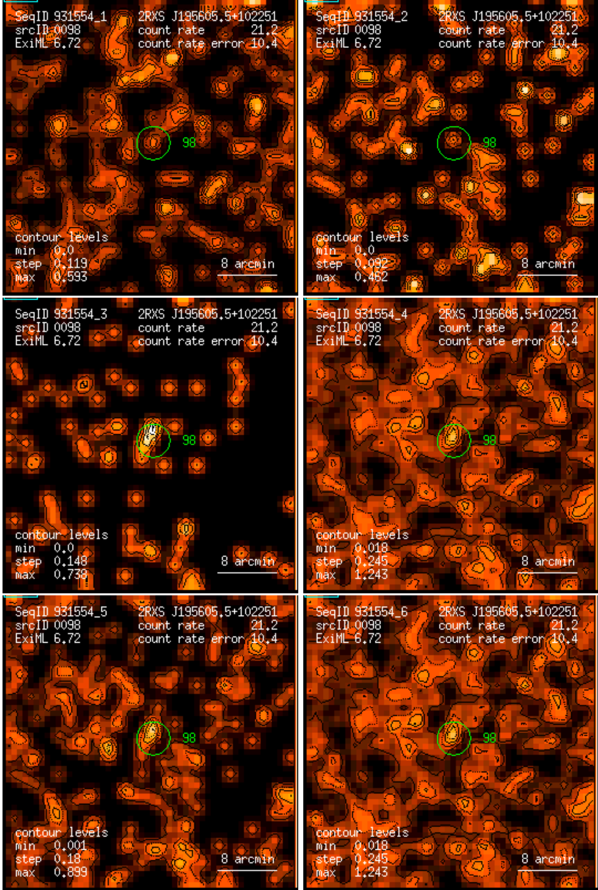
Figure 98: RASS 931554: detection 0098: band rate images, Gaussian filter: (1) PSPC channels 11 – 41, (2) 52 – 90, (3) 91 – 201, (4) 11 – 235, (5) 52 – 201, (6) 11 – 201. Broad band rates in counts/ks. Band rate contour levels in counts/ks/arcmin 2 .
