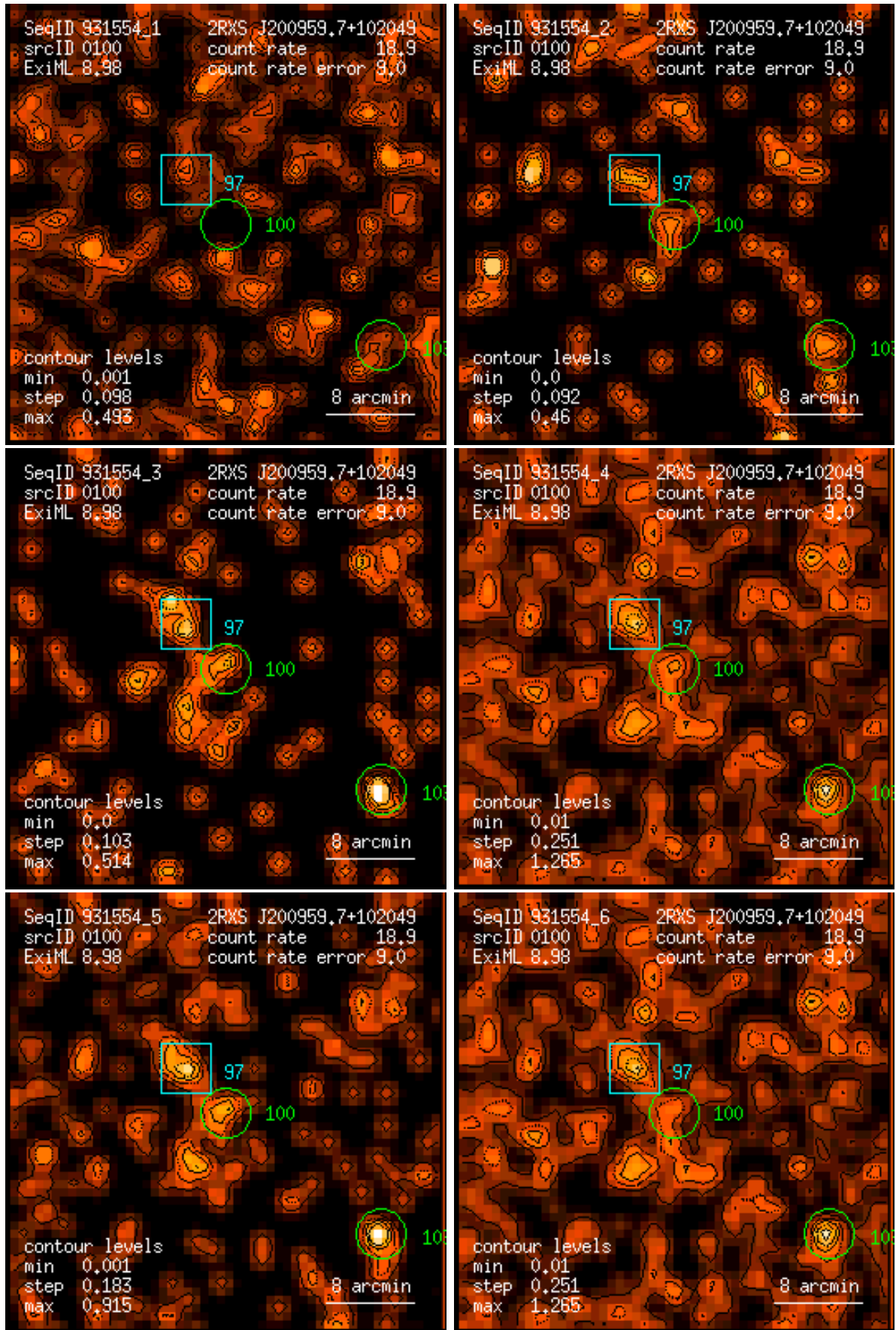
Figure 100: RASS 931554: detection 0100: band rate images, Gaussian filter: (1) PSPC channels 11 – 41, (2) 52 – 90, (3) 91 – 201, (4) 11 – 235, (5) 52 – 201, (6) 11 – 201. Broad band rates in counts/ks. Band rate contour levels in counts/ks/arcmin 2 .
