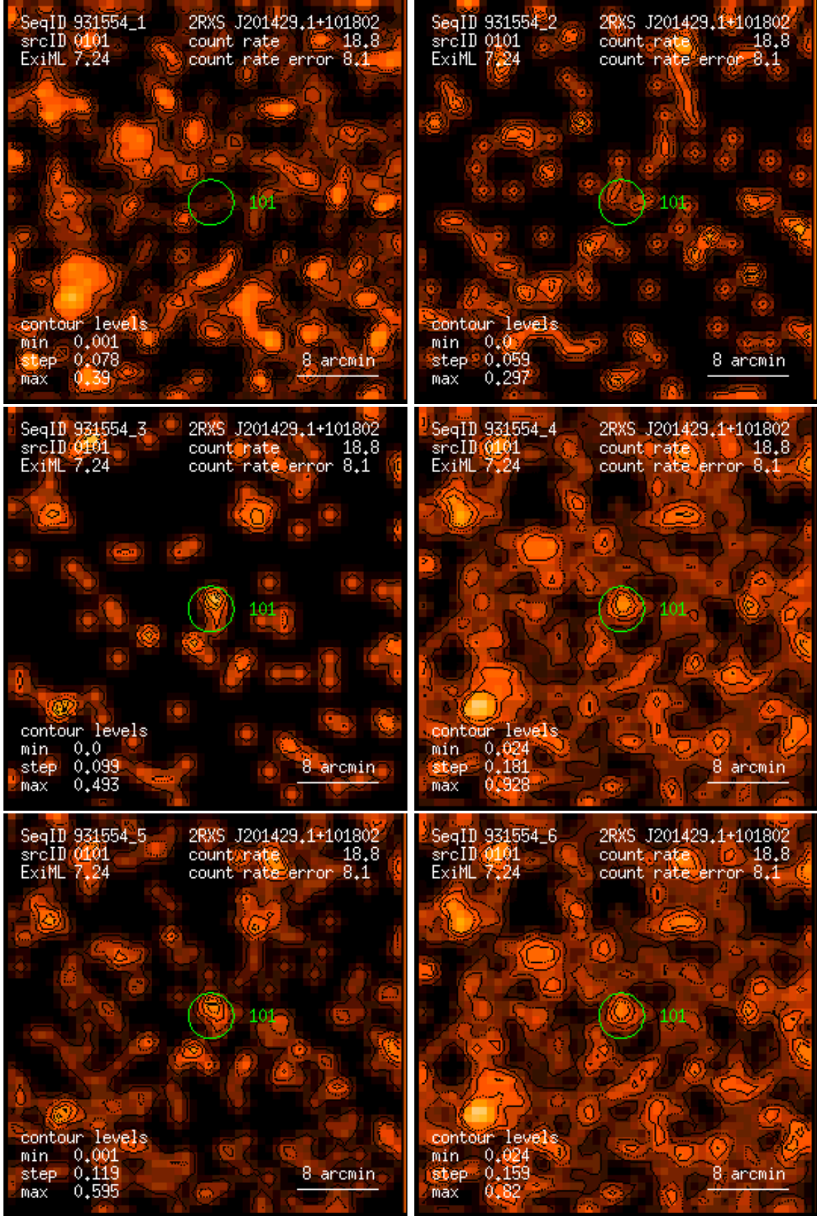
Figure 101: RASS 931554: detection 0101: band rate images, Gaussian filter: (1) PSPC channels 11 – 41, (2) 52 – 90, (3) 91 – 201, (4) 11 – 235, (5) 52 – 201, (6) 11 – 201. Broad band rates in counts/ks. Band rate contour levels in counts/ks/arcmin 2 .
