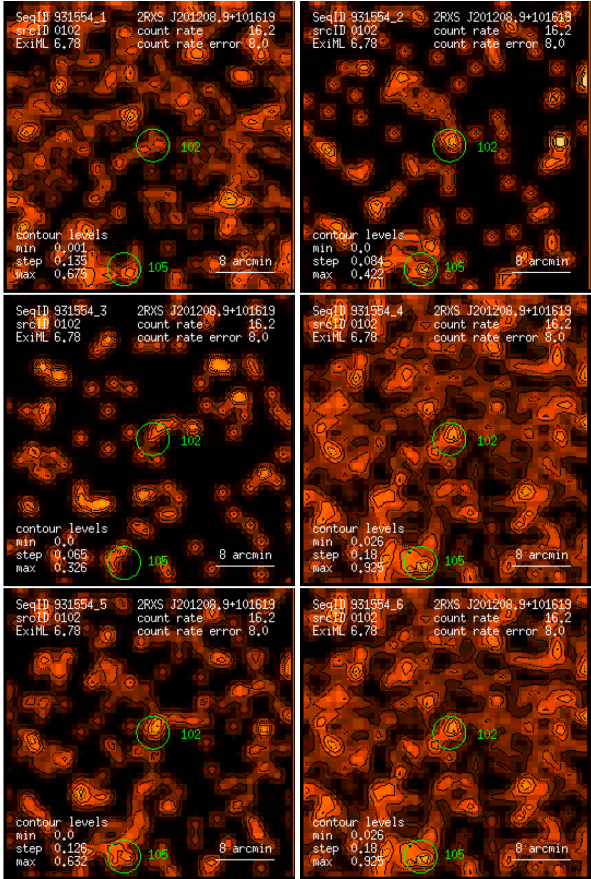
Figure 102: RASS 931554: detection 0102: band rate images, Gaussian filter: (1) PSPC channels 11 – 41, (2) 52 – 90, (3) 91 – 201, (4) 11 – 235, (5) 52 – 201, (6) 11 – 201. Broad band rates in counts/ks. Band rate contour levels in counts/ks/arcmin 2 .
