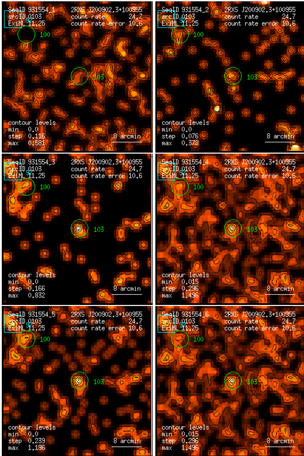
Figure 103: RASS 931554: detection 0103: band rate images, Gaussian filter: (1) PSPC channels 11 – 41, (2) 52 – 90, (3) 91 – 201, (4) 11 – 235, (5) 52 – 201, (6) 11 – 201. Broad band rates in counts/ks. Band rate contour levels in counts/ks/arcmin 2 .
