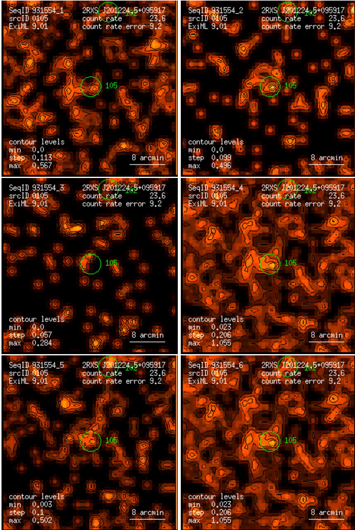
Figure 105: RASS 931554: detection 0105: band rate images, Gaussian filter: (1) PSPC channels 11 – 41, (2) 52 – 90, (3) 91 – 201, (4) 11 – 235, (5) 52 – 201, (6) 11 – 201. Broad band rates in counts/ks. Band rate contour levels in counts/ks/arcmin 2 .
