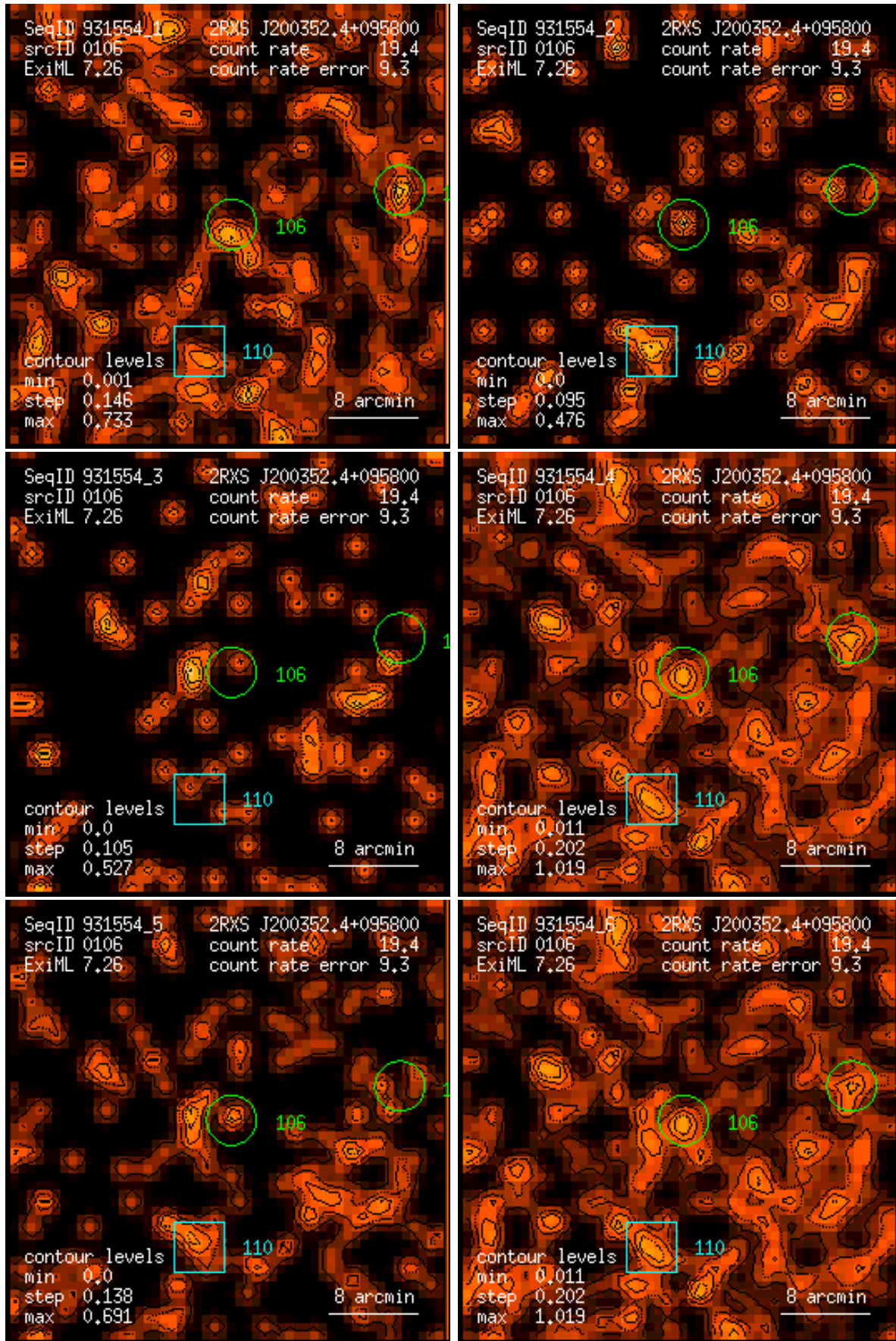
Figure 106: RASS 931554: detection 0106: band rate images, Gaussian filter: (1) PSPC channels 11 – 41, (2) 52 – 90, (3) 91 – 201, (4) 11 – 235, (5) 52 – 201, (6) 11 – 201. Broad band rates in counts/ks. Band rate contour levels in counts/ks/arcmin 2 .
