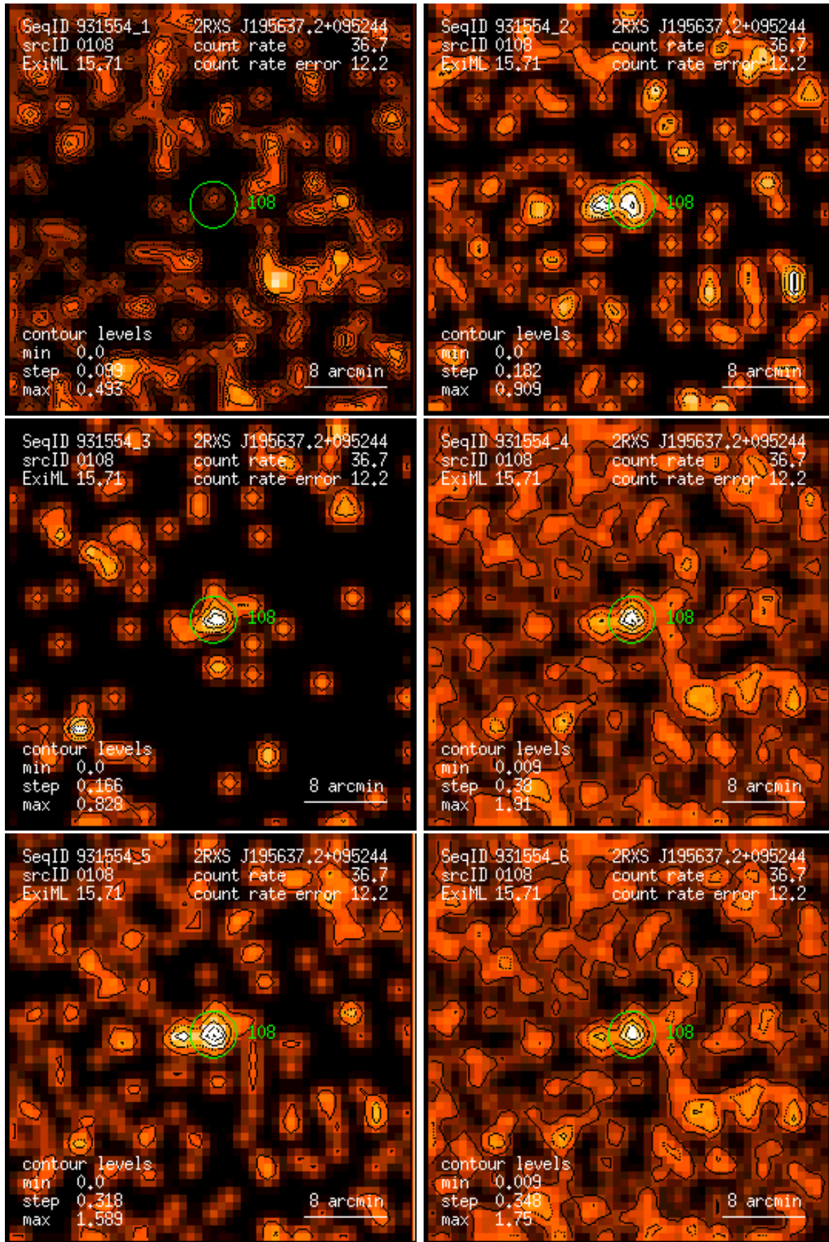
Figure 108: RASS 931554: detection 0108: band rate images, Gaussian filter: (1) PSPC channels 11 – 41, (2) 52 – 90, (3) 91 – 201, (4) 11 – 235, (5) 52 – 201, (6) 11 – 201. Broad band rates in counts/ks. Band rate contour levels in counts/ks/arcmin 2 .
