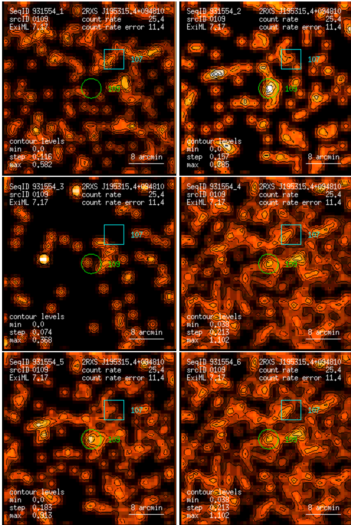
Figure 109: RASS 931554: detection 0109: band rate images, Gaussian filter: (1) PSPC channels 11 – 41, (2) 52 – 90, (3) 91 – 201, (4) 11 – 235, (5) 52 – 201, (6) 11 – 201. Broad band rates in counts/ks. Band rate contour levels in counts/ks/arcmin 2 .
