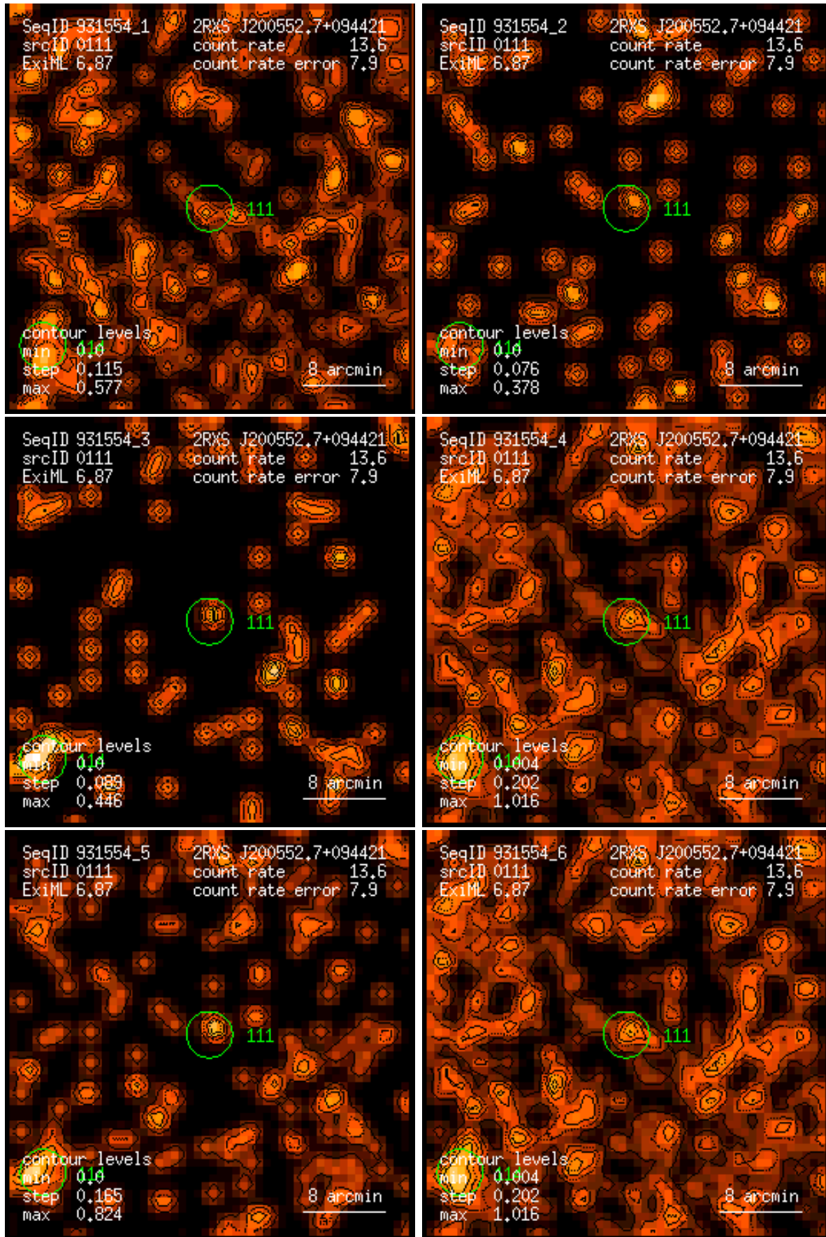
Figure 111: RASS 931554: detection 0111: band rate images, Gaussian filter: (1) PSPC channels 11 – 41, (2) 52 – 90, (3) 91 – 201, (4) 11 – 235, (5) 52 – 201, (6) 11 – 201. Broad band rates in counts/ks. Band rate contour levels in counts/ks/arcmin 2 .
