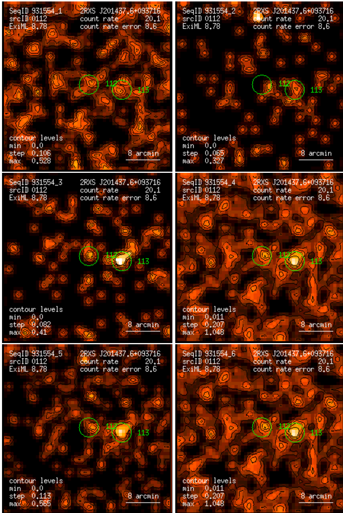
Figure 112: RASS 931554: detection 0112: band rate images, Gaussian filter: (1) PSPC channels 11 – 41, (2) 52 – 90, (3) 91 – 201, (4) 11 – 235, (5) 52 – 201, (6) 11 – 201. Broad band rates in counts/ks. Band rate contour levels in counts/ks/arcmin 2 .
