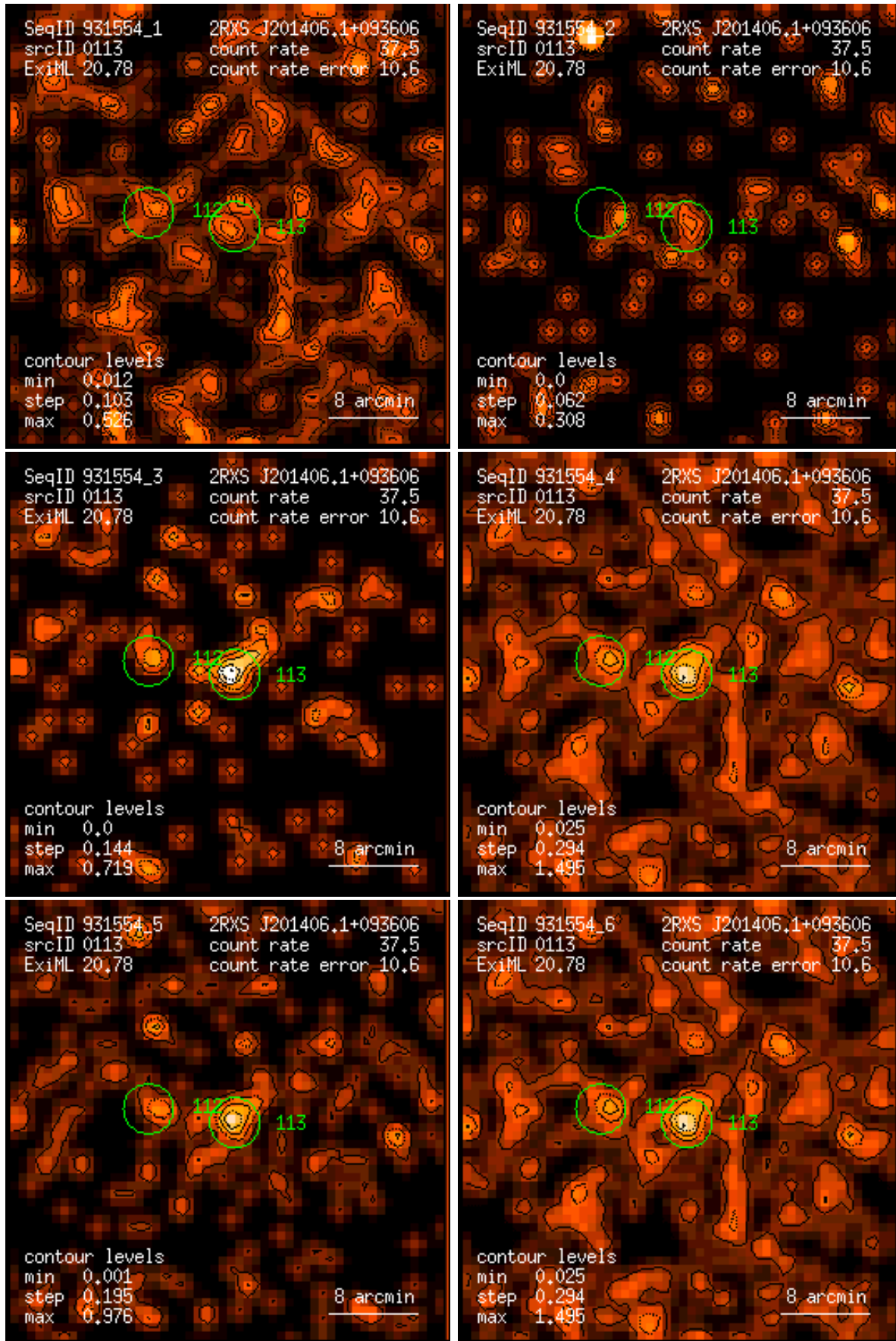
Figure 113: RASS 931554: detection 0113: band rate images, Gaussian filter: (1) PSPC channels 11 – 41, (2) 52 – 90, (3) 91 – 201, (4) 11 – 235, (5) 52 – 201, (6) 11 – 201. Broad band rates in counts/ks. Band rate contour levels in counts/ks/arcmin 2 .
