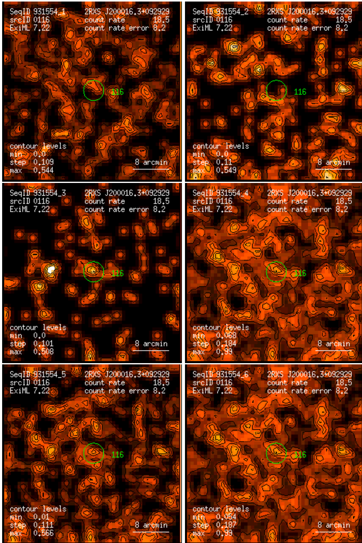
Figure 116: RASS 931554: detection 0116: band rate images, Gaussian filter: (1) PSPC channels 11 – 41, (2) 52 – 90, (3) 91 – 201, (4) 11 – 235, (5) 52 – 201, (6) 11 – 201. Broad band rates in counts/ks. Band rate contour levels in counts/ks/arcmin 2 .
