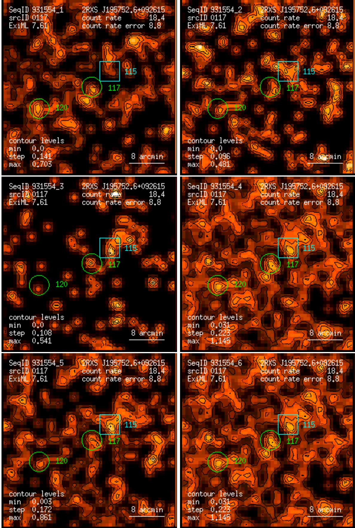
Figure 117: RASS 931554: detection 0117: band rate images, Gaussian filter: (1) PSPC channels 11 – 41, (2) 52 – 90, (3) 91 – 201, (4) 11 – 235, (5) 52 – 201, (6) 11 – 201. Broad band rates in counts/ks. Band rate contour levels in counts/ks/arcmin 2 .
