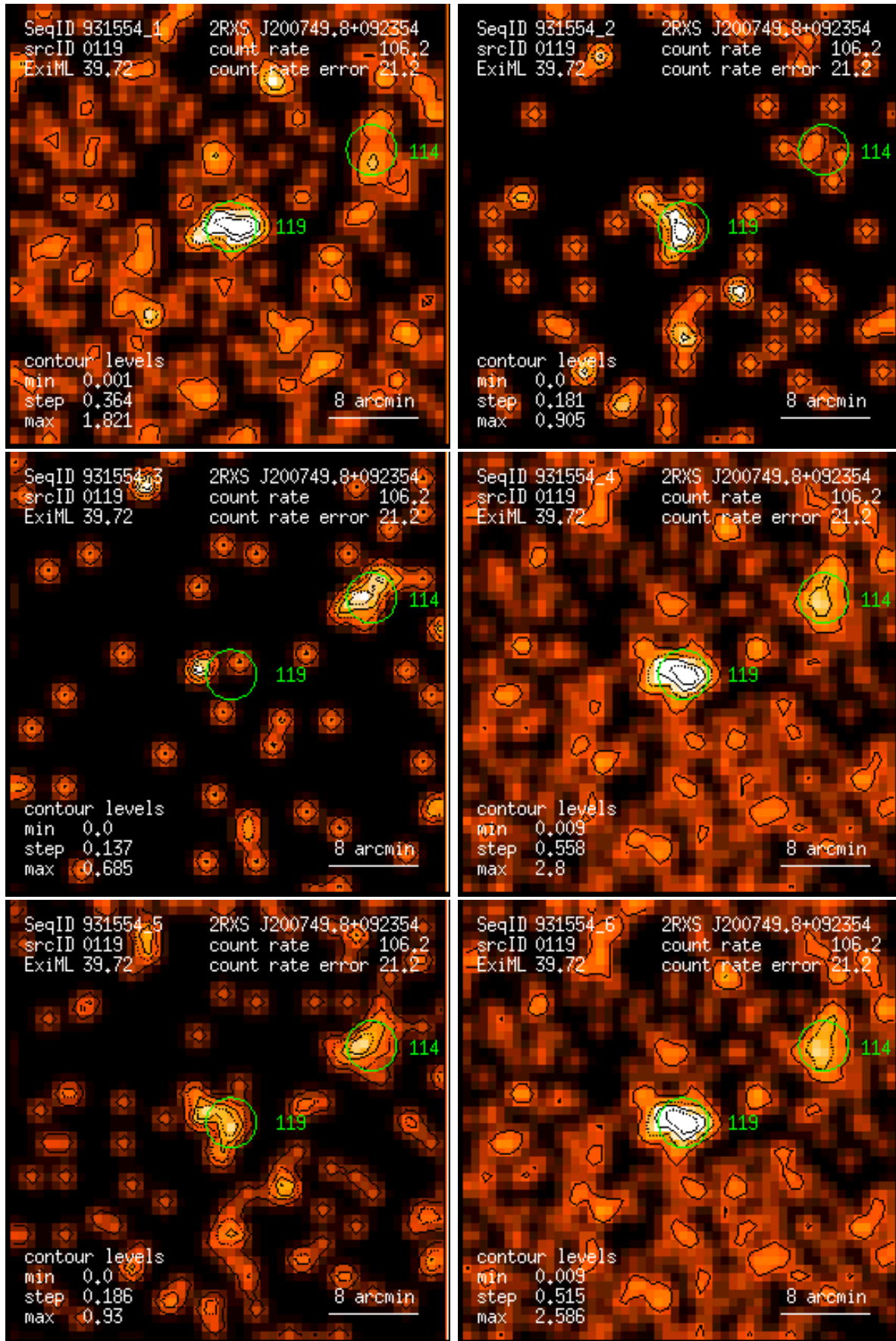
Figure 119: RASS 931554: detection 0119: band rate images, Gaussian filter: (1) PSPC channels 11 – 41, (2) 52 – 90, (3) 91 – 201, (4) 11 – 235, (5) 52 – 201, (6) 11 – 201. Broad band rates in counts/ks. Band rate contour levels in counts/ks/arcmin 2 .
