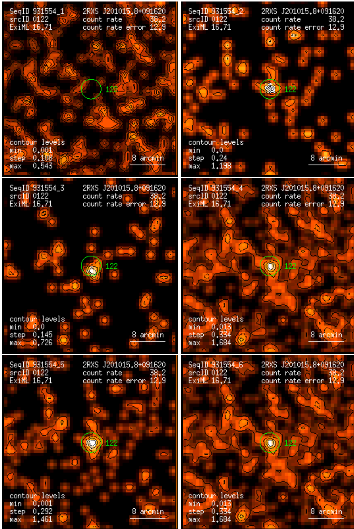
Figure 122: RASS 931554: detection 0122: band rate images, Gaussian filter: (1) PSPC channels 11 – 41, (2) 52 – 90, (3) 91 – 201, (4) 11 – 235, (5) 52 – 201, (6) 11 – 201. Broad band rates in counts/ks. Band rate contour levels in counts/ks/arcmin 2 .
