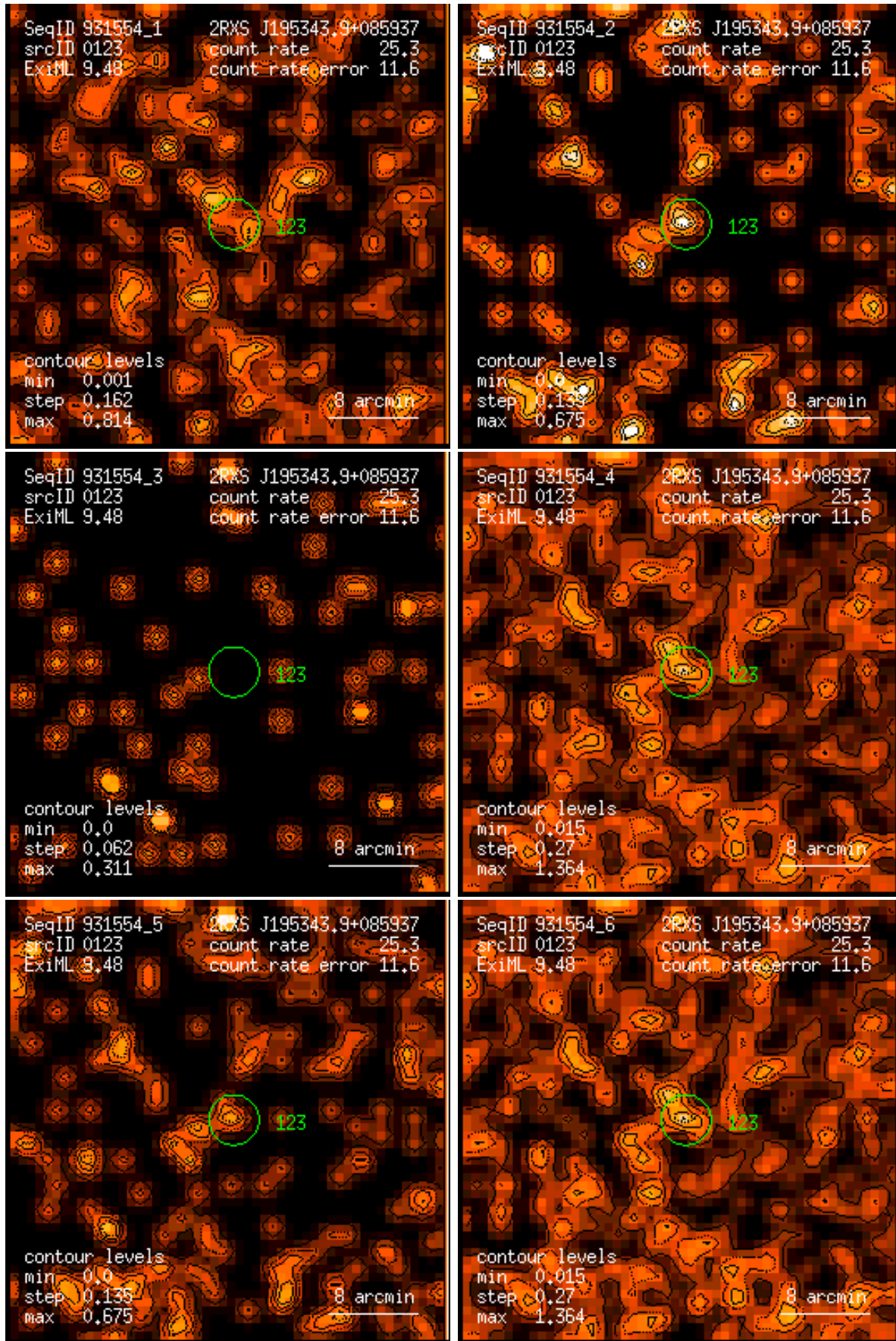
Figure 123: RASS 931554: detection 0123: band rate images, Gaussian filter: (1) PSPC channels 11 – 41, (2) 52 – 90, (3) 91 – 201, (4) 11 – 235, (5) 52 – 201, (6) 11 – 201. Broad band rates in counts/ks. Band rate contour levels in counts/ks/arcmin 2 .
