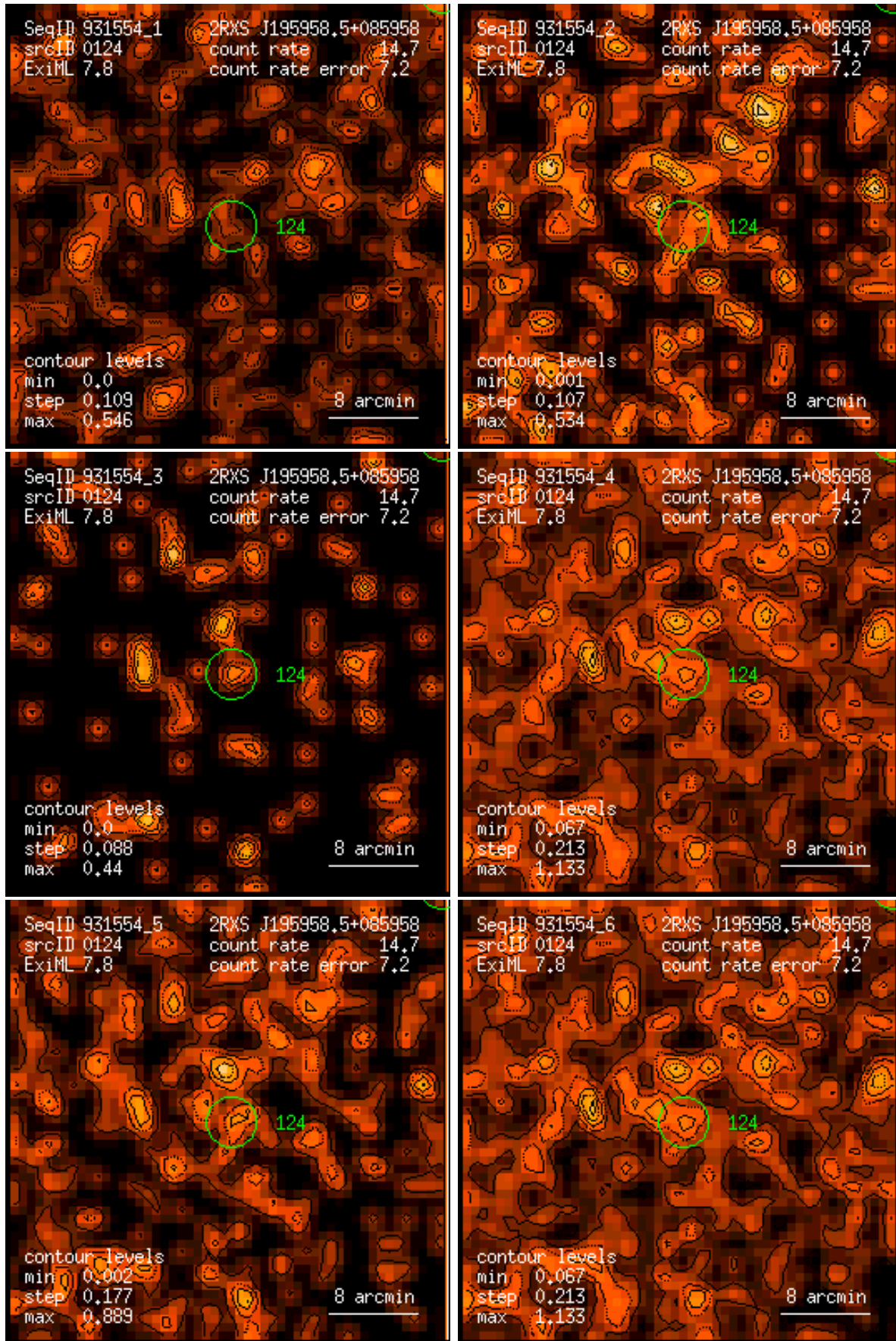
Figure 124: RASS 931554: detection 0124: band rate images, Gaussian filter: (1) PSPC channels 11 – 41, (2) 52 – 90, (3) 91 – 201, (4) 11 – 235, (5) 52 – 201, (6) 11 – 201. Broad band rates in counts/ks. Band rate contour levels in counts/ks/arcmin 2 .
