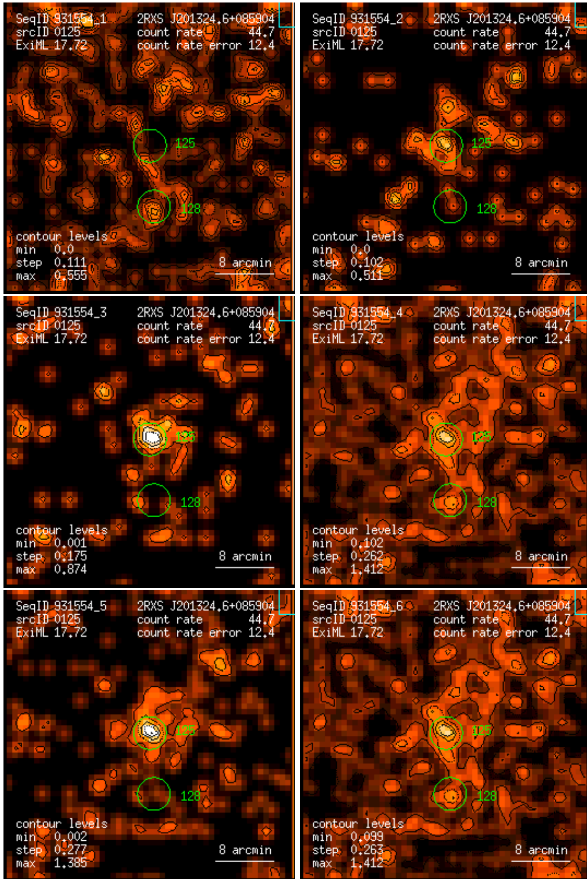
Figure 125: RASS 931554: detection 0125: band rate images, Gaussian filter: (1) PSPC channels 11 – 41, (2) 52 – 90, (3) 91 – 201, (4) 11 – 235, (5) 52 – 201, (6) 11 – 201. Broad band rates in counts/ks. Band rate contour levels in counts/ks/arcmin 2 .
