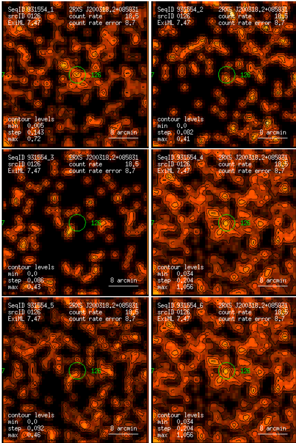
Figure 126: RASS 931554: detection 0126: band rate images, Gaussian filter: (1) PSPC channels 11 – 41, (2) 52 – 90, (3) 91 – 201, (4) 11 – 235, (5) 52 – 201, (6) 11 – 201. Broad band rates in counts/ks. Band rate contour levels in counts/ks/arcmin 2 .
