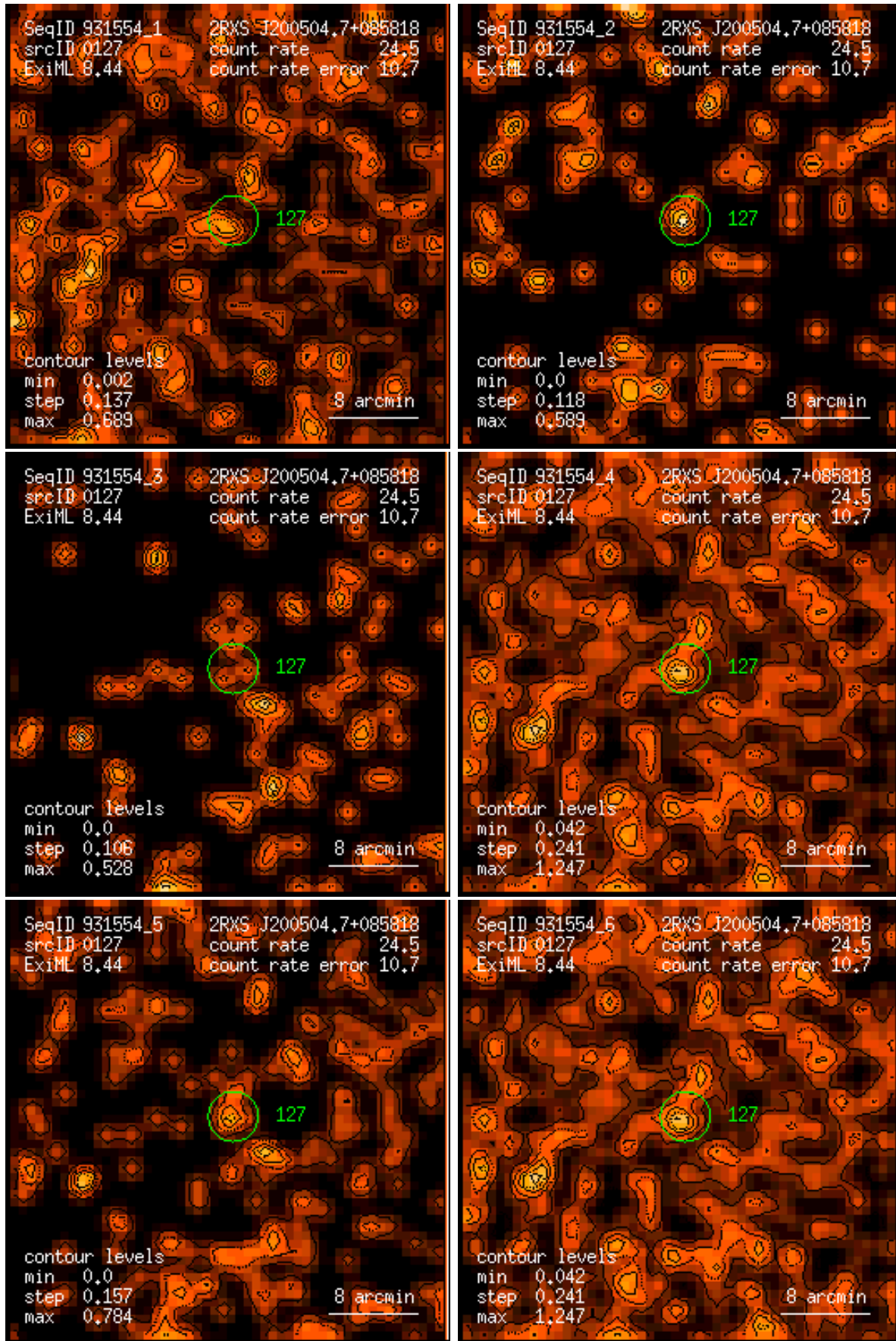
Figure 127: RASS 931554: detection 0127: band rate images, Gaussian filter: (1) PSPC channels 11 – 41, (2) 52 – 90, (3) 91 – 201, (4) 11 – 235, (5) 52 – 201, (6) 11 – 201. Broad band rates in counts/ks. Band rate contour levels in counts/ks/arcmin 2 .
