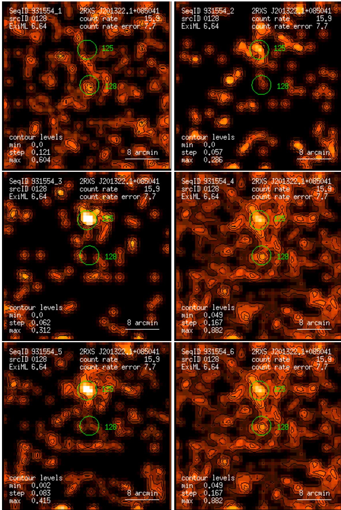
Figure 128: RASS 931554: detection 0128: band rate images, Gaussian filter: (1) PSPC channels 11 – 41, (2) 52 – 90, (3) 91 – 201, (4) 11 – 235, (5) 52 – 201, (6) 11 – 201. Broad band rates in counts/ks. Band rate contour levels in counts/ks/arcmin 2 .
