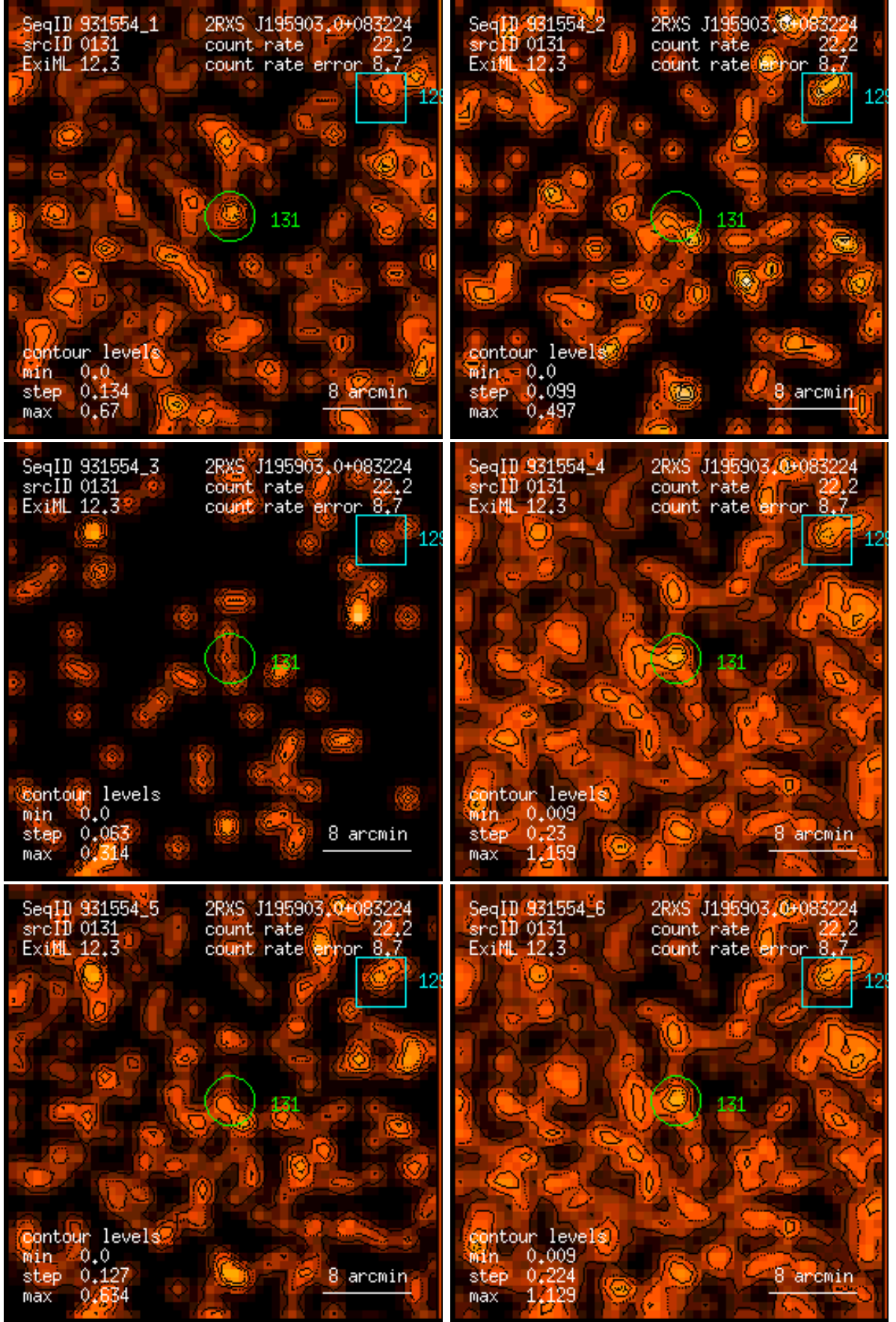
Figure 131: RASS 931554: detection 0131: band rate images, Gaussian filter: (1) PSPC channels 11 – 41, (2) 52 – 90, (3) 91 – 201, (4) 11 – 235, (5) 52 – 201, (6) 11 – 201. Broad band rates in counts/ks. Band rate contour levels in counts/ks/arcmin 2 .
