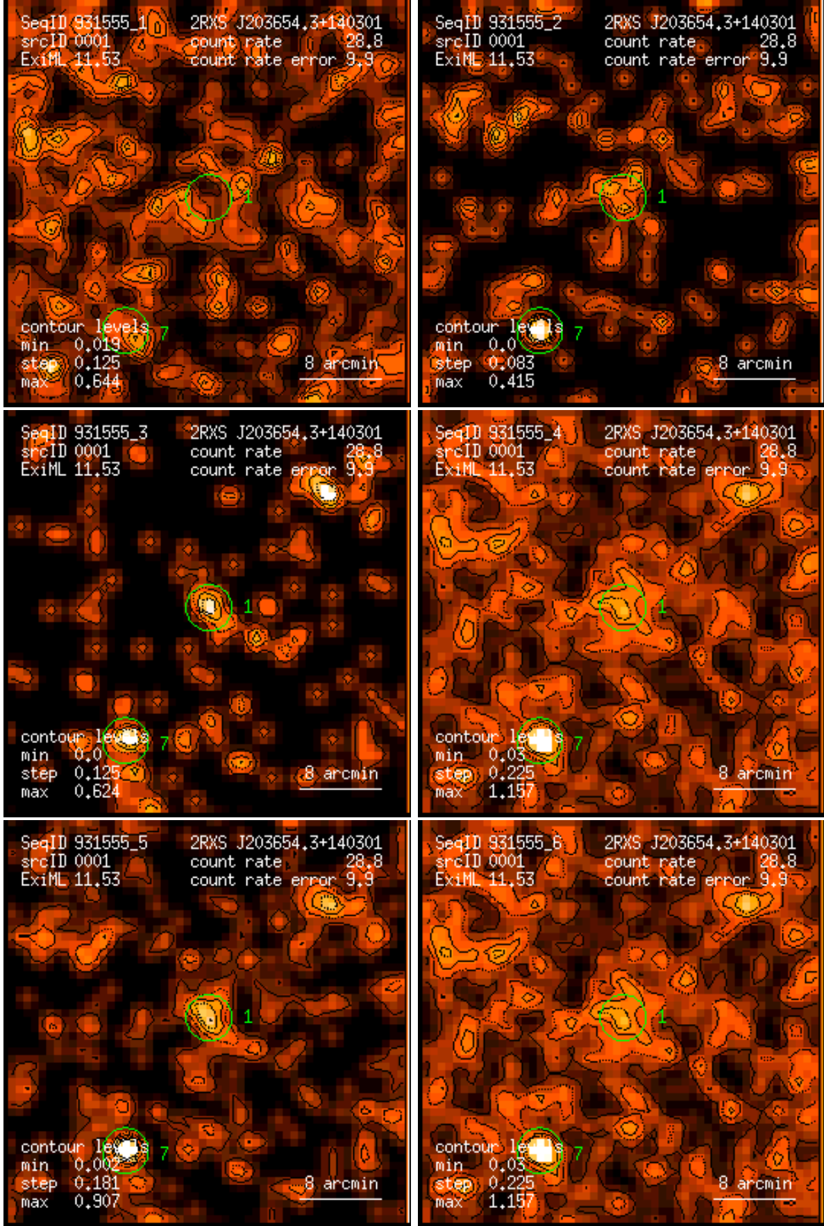
Figure 1: RASS 931555: detection 0001: band rate images, Gaussian filter: (1) PSPC channels 11 – 41, (2) 52 – 90, (3) 91 – 201, (4) 11 – 235, (5) 52 – 201, (6) 11 – 201. Broad band rates in counts/ks. Band rate contour levels in counts/ks/arcmin 2 .
