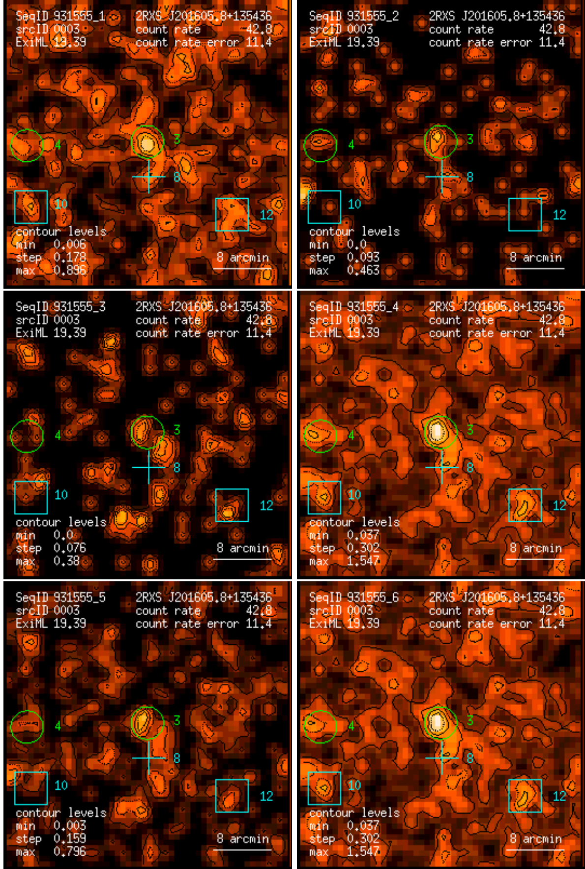
Figure 3: RASS 931555: detection 0003: band rate images, Gaussian filter: (1) PSPC channels 11 – 41, (2) 52 – 90, (3) 91 – 201, (4) 11 – 235, (5) 52 – 201, (6) 11 – 201. Broad band rates in counts/ks. Band rate contour levels in counts/ks/arcmin 2 .
