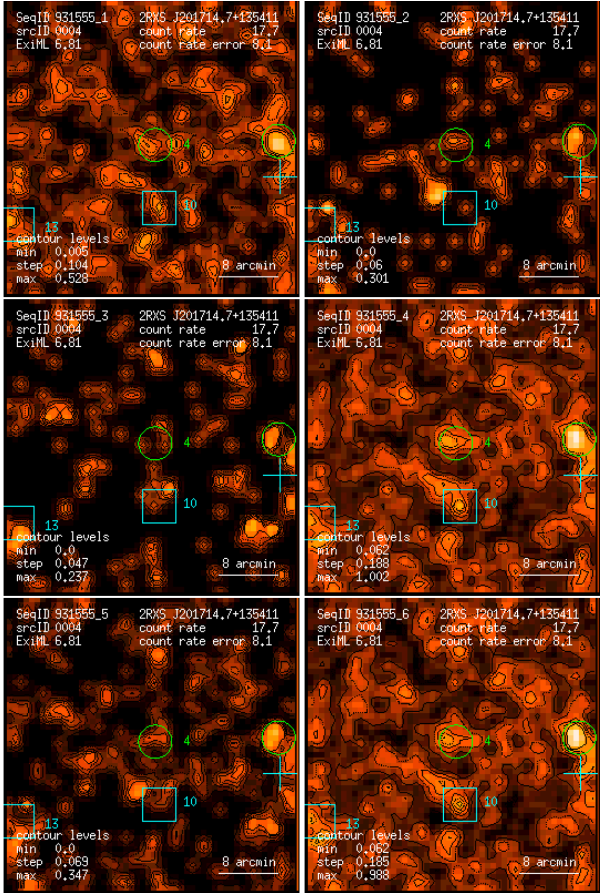
Figure 4: RASS 931555: detection 0004: band rate images, Gaussian filter: (1) PSPC channels 11 – 41, (2) 52 – 90, (3) 91 – 201, (4) 11 – 235, (5) 52 – 201, (6) 11 – 201. Broad band rates in counts/ks. Band rate contour levels in counts/ks/arcmin 2 .
