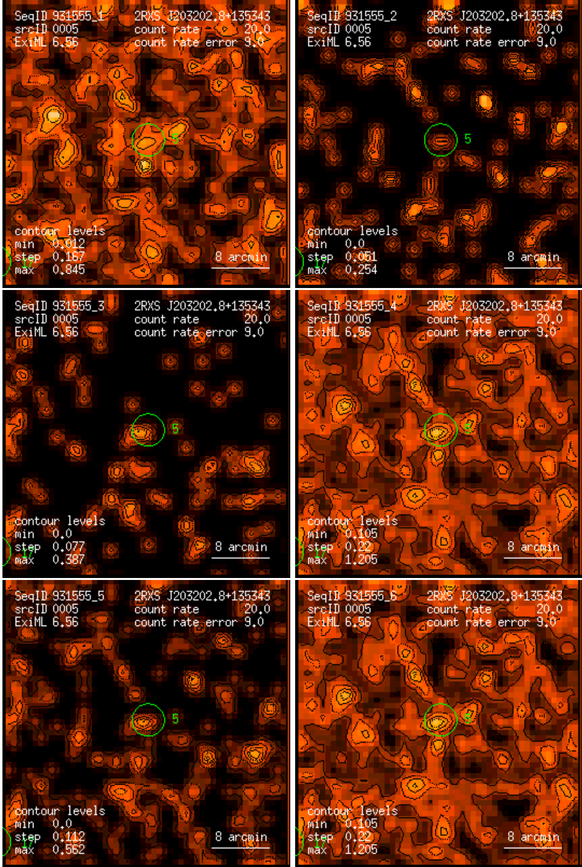
Figure 5: RASS 931555: detection 0005: band rate images, Gaussian filter: (1) PSPC channels 11 – 41, (2) 52 – 90, (3) 91 – 201, (4) 11 – 235, (5) 52 – 201, (6) 11 – 201. Broad band rates in counts/ks. Band rate contour levels in counts/ks/arcmin 2 .
