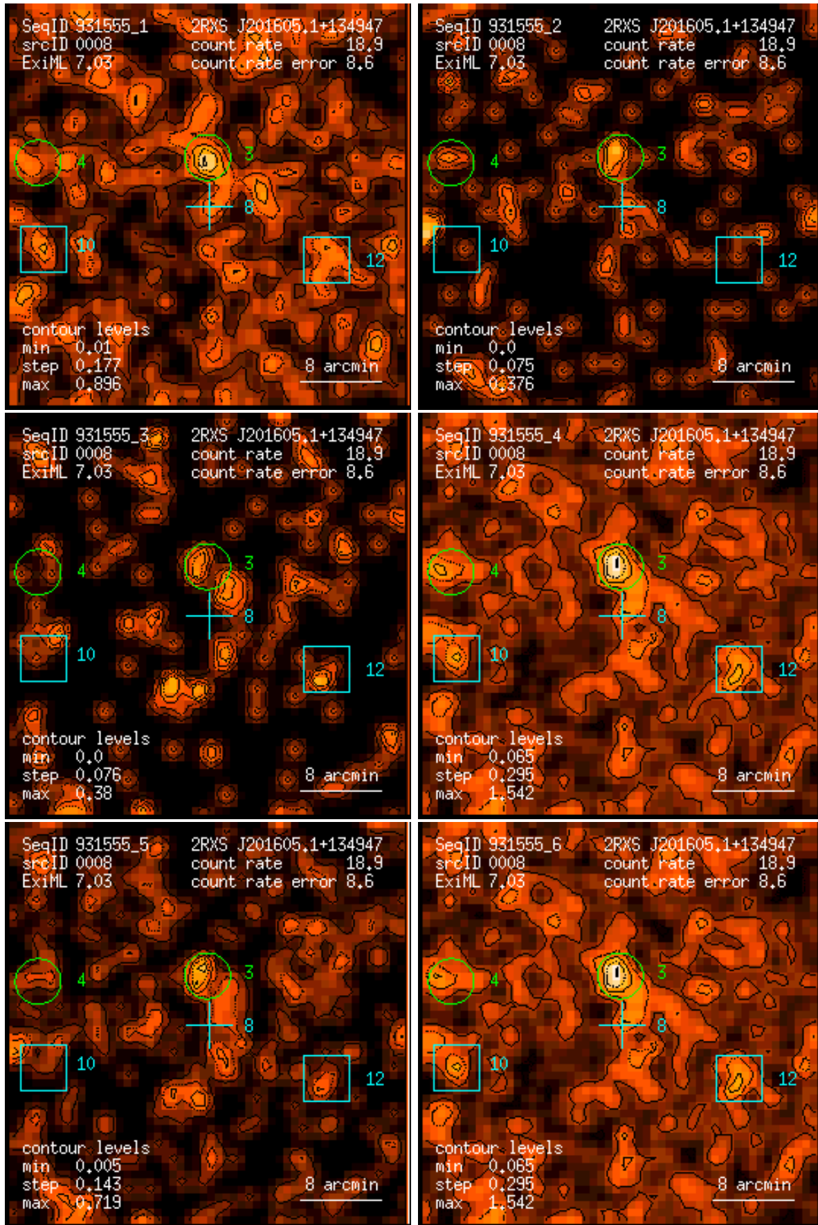
Figure 8: RASS 931555: detection 0008: band rate images, Gaussian filter: (1) PSPC channels 11 – 41, (2) 52 – 90, (3) 91 – 201, (4) 11 – 235, (5) 52 – 201, (6) 11 – 201. Broad band rates in counts/ks. Band rate contour levels in counts/ks/arcmin 2 .
