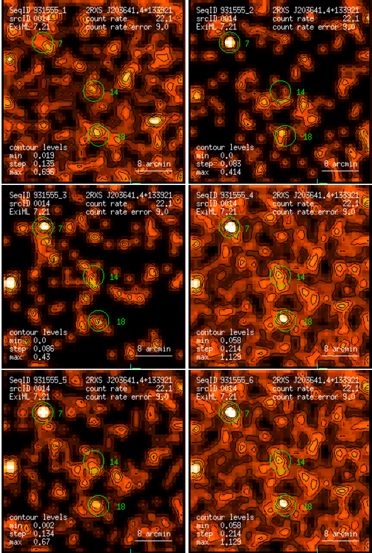
Figure 14: RASS 931555: detection 0014: band rate images, Gaussian filter: (1) PSPC channels 11 – 41, (2) 52 – 90, (3) 91 – 201, (4) 11 – 235, (5) 52 – 201, (6) 11 – 201. Broad band rates in counts/ks. Band rate contour levels in counts/ks/arcmin 2 .
