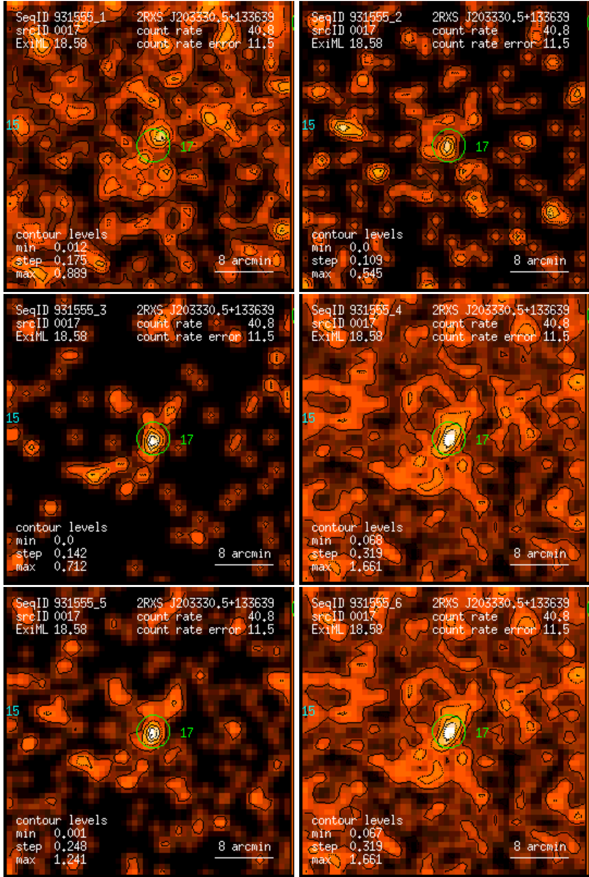
Figure 17: RASS 931555: detection 0017: band rate images, Gaussian filter: (1) PSPC channels 11 – 41, (2) 52 – 90, (3) 91 – 201, (4) 11 – 235, (5) 52 – 201, (6) 11 – 201. Broad band rates in counts/ks. Band rate contour levels in counts/ks/arcmin 2 .
