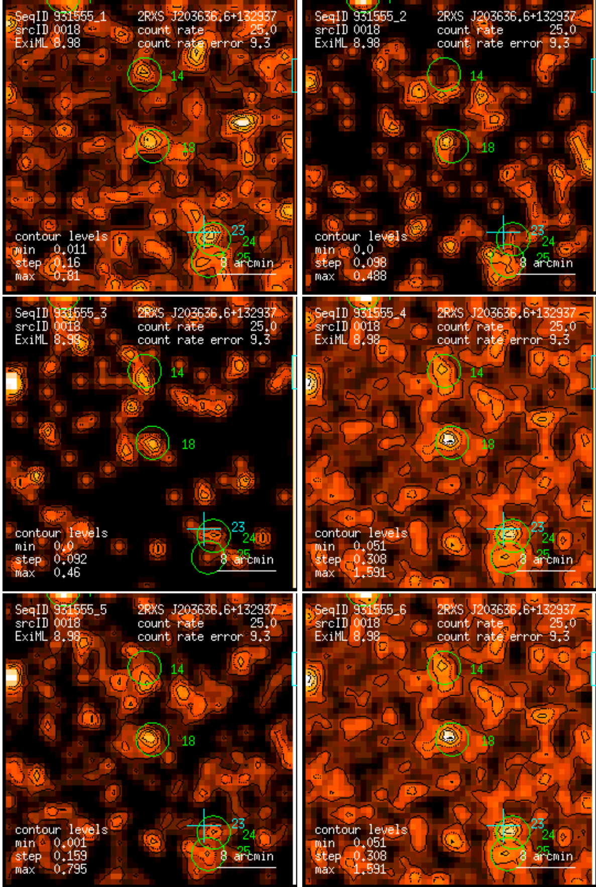
Figure 18: RASS 931555: detection 0018: band rate images, Gaussian filter: (1) PSPC channels 11 – 41, (2) 52 – 90, (3) 91 – 201, (4) 11 – 235, (5) 52 – 201, (6) 11 – 201. Broad band rates in counts/ks. Band rate contour levels in counts/ks/arcmin 2 .
