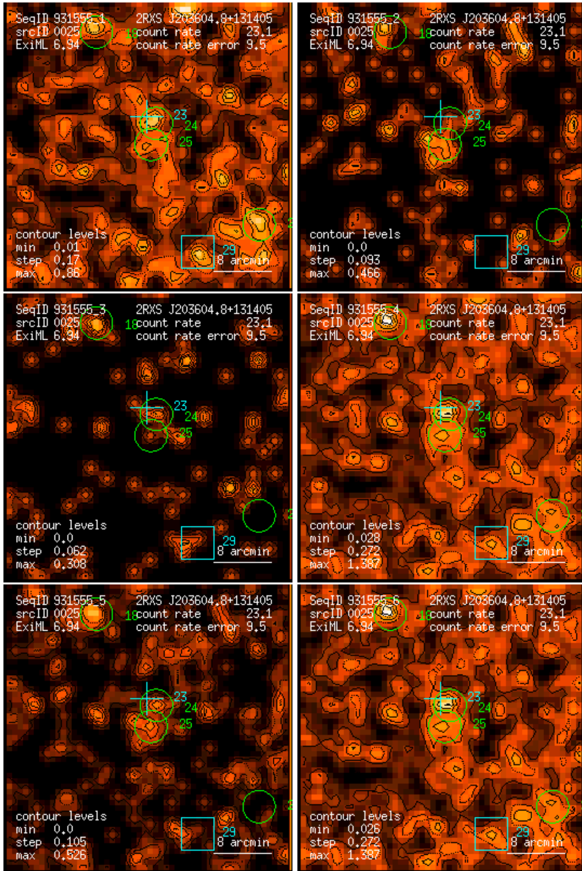
Figure 25: RASS 931555: detection 0025: band rate images, Gaussian filter: (1) PSPC channels 11 – 41, (2) 52 – 90, (3) 91 – 201, (4) 11 – 235, (5) 52 – 201, (6) 11 – 201. Broad band rates in counts/ks. Band rate contour levels in counts/ks/arcmin 2 .
