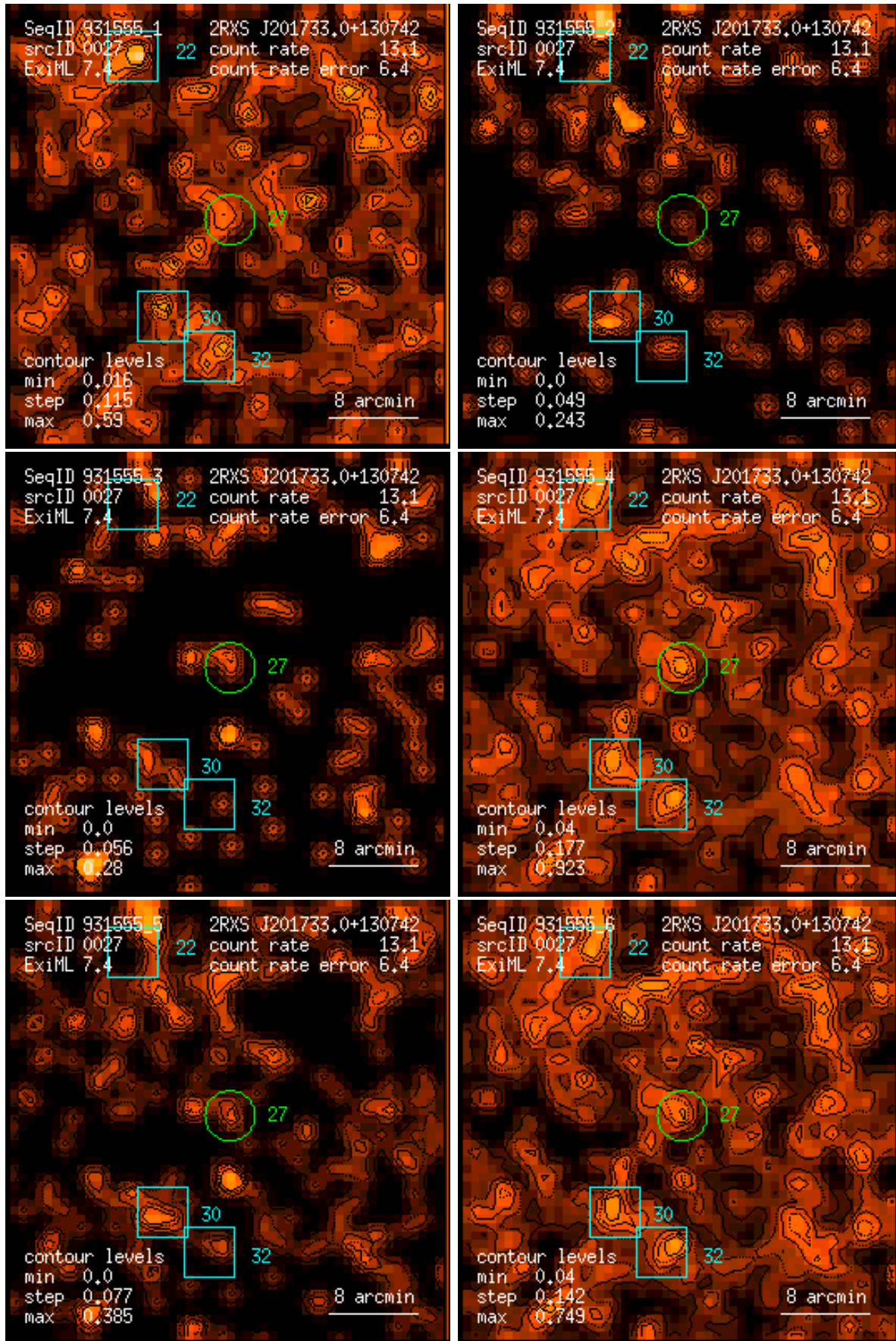
Figure 27: RASS 931555: detection 0027: band rate images, Gaussian filter: (1) PSPC channels 11 – 41, (2) 52 – 90, (3) 91 – 201, (4) 11 – 235, (5) 52 – 201, (6) 11 – 201. Broad band rates in counts/ks. Band rate contour levels in counts/ks/arcmin 2 .
