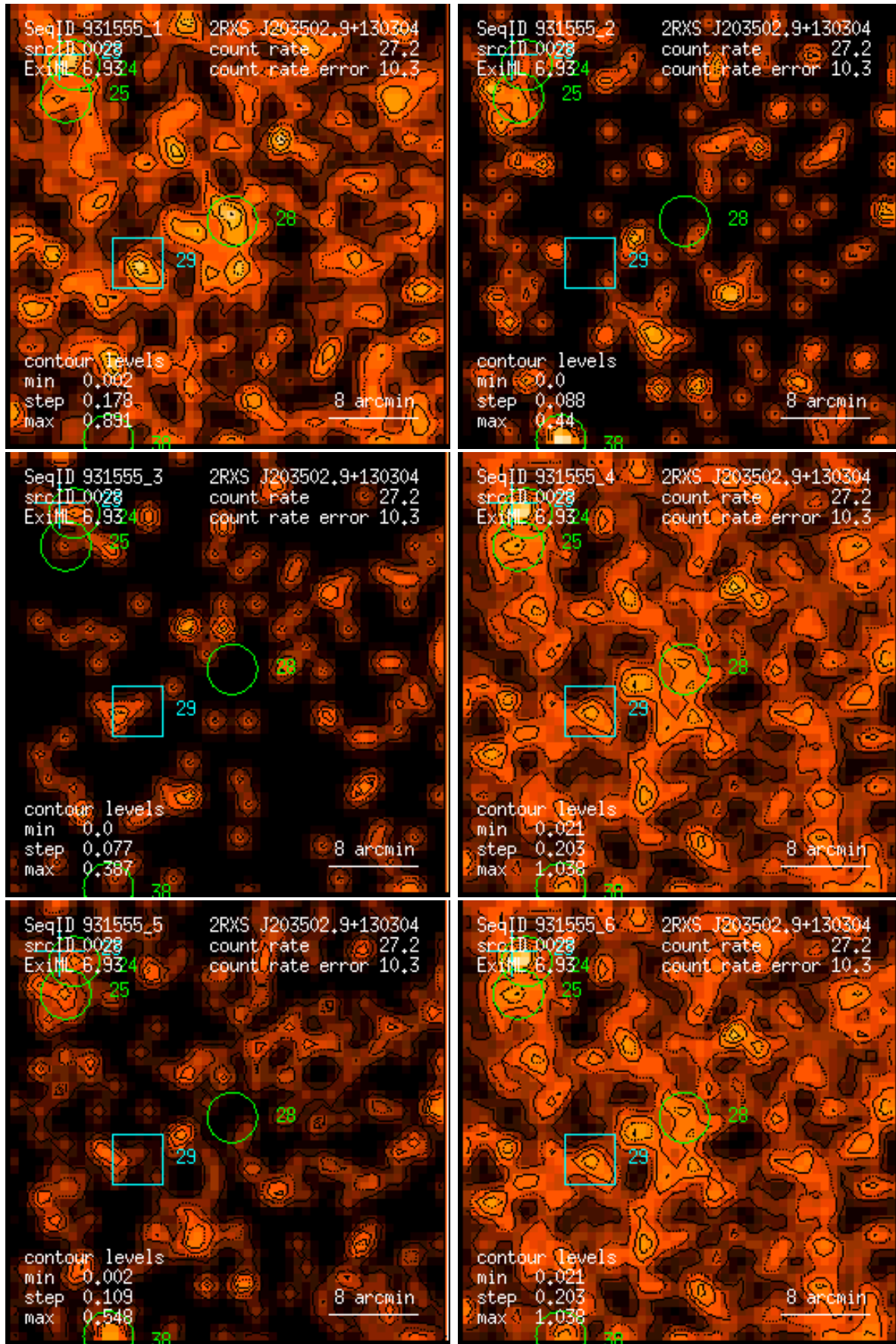
Figure 28: RASS 931555: detection 0028: band rate images, Gaussian filter: (1) PSPC channels 11 – 41, (2) 52 – 90, (3) 91 – 201, (4) 11 – 235, (5) 52 – 201, (6) 11 – 201. Broad band rates in counts/ks. Band rate contour levels in counts/ks/arcmin 2 .
