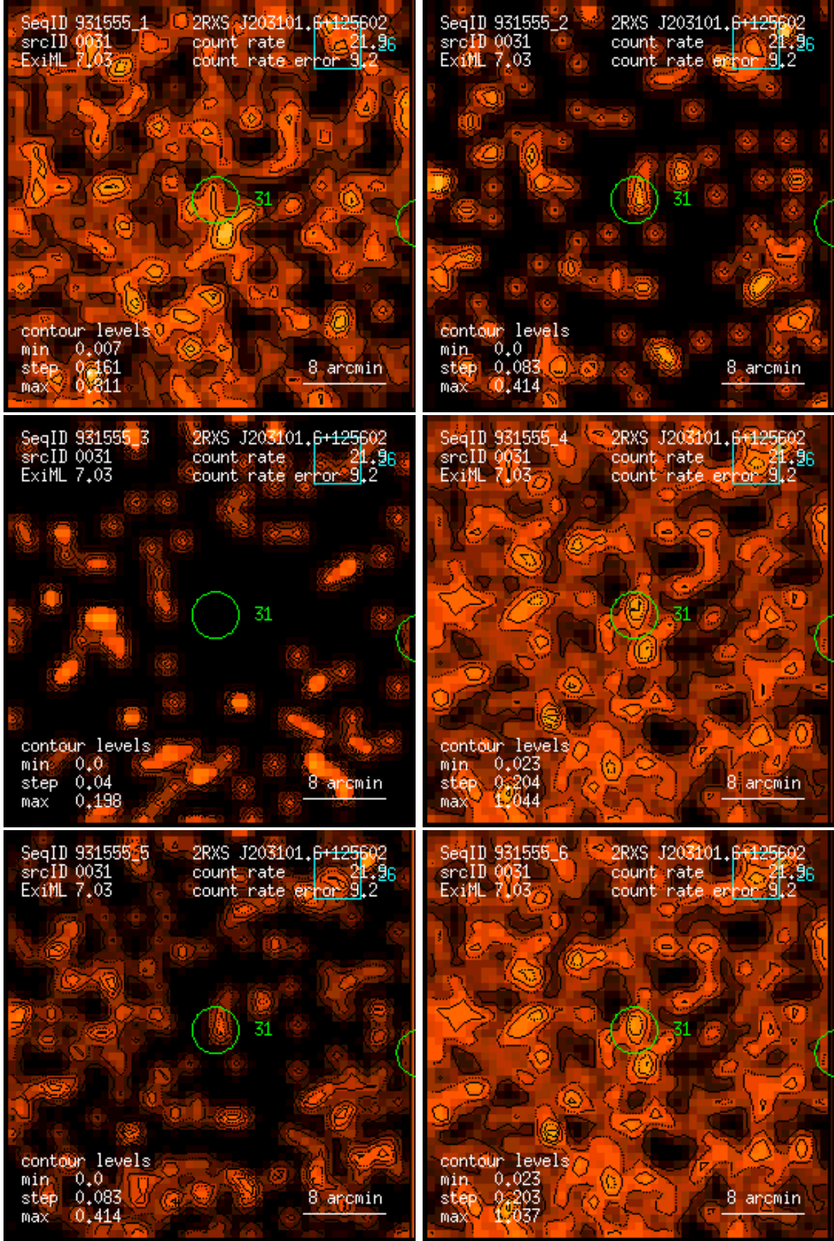
Figure 31: RASS 931555: detection 0031: band rate images, Gaussian filter: (1) PSPC channels 11 – 41, (2) 52 – 90, (3) 91 – 201, (4) 11 – 235, (5) 52 – 201, (6) 11 – 201. Broad band rates in counts/ks. Band rate contour levels in counts/ks/arcmin 2 .
