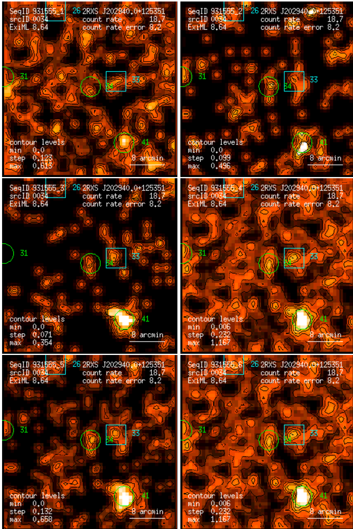
Figure 34: RASS 931555: detection 0034: band rate images, Gaussian filter: (1) PSPC channels 11 – 41, (2) 52 – 90, (3) 91 – 201, (4) 11 – 235, (5) 52 – 201, (6) 11 – 201. Broad band rates in counts/ks. Band rate contour levels in counts/ks/arcmin 2 .
