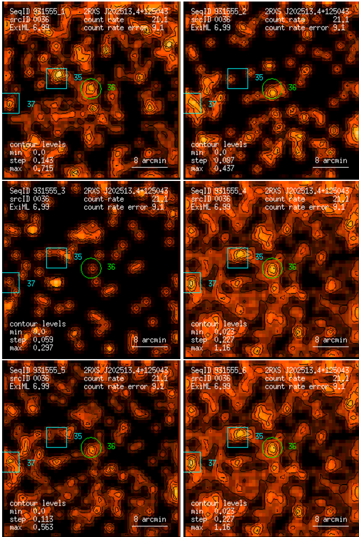
Figure 36: RASS 931555: detection 0036: band rate images, Gaussian filter: (1) PSPC channels 11 – 41, (2) 52 – 90, (3) 91 – 201, (4) 11 – 235, (5) 52 – 201, (6) 11 – 201. Broad band rates in counts/ks. Band rate contour levels in counts/ks/arcmin 2 .
