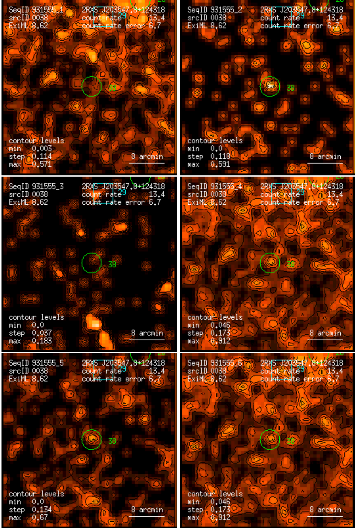
Figure 38: RASS 931555: detection 0038: band rate images, Gaussian filter: (1) PSPC channels 11 – 41, (2) 52 – 90, (3) 91 – 201, (4) 11 – 235, (5) 52 – 201, (6) 11 – 201. Broad band rates in counts/ks. Band rate contour levels in counts/ks/arcmin 2 .
