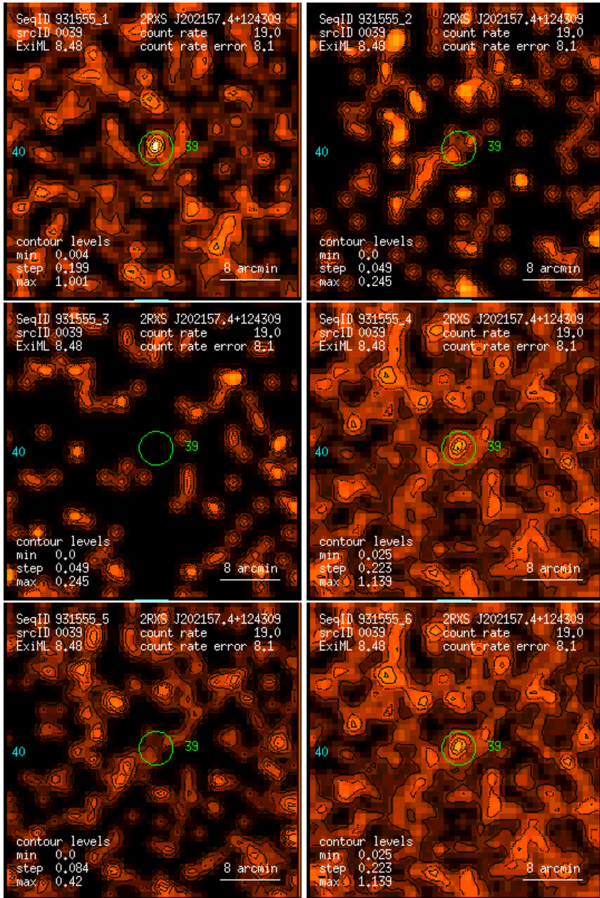
Figure 39: RASS 931555: detection 0039: band rate images, Gaussian filter: (1) PSPC channels 11 – 41, (2) 52 – 90, (3) 91 – 201, (4) 11 – 235, (5) 52 – 201, (6) 11 – 201. Broad band rates in counts/ks. Band rate contour levels in counts/ks/arcmin 2 .
